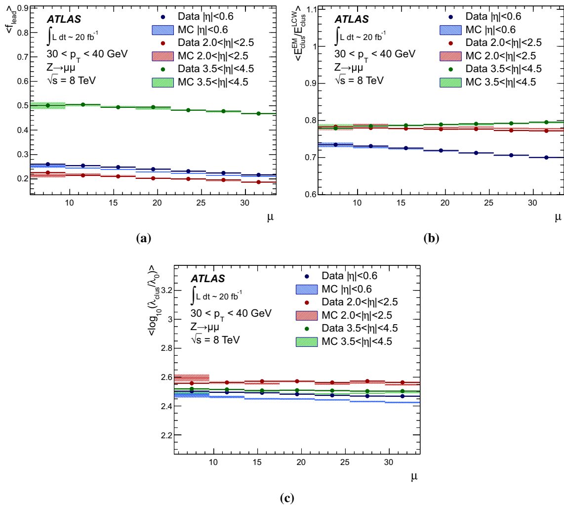
Fig. 40 The pile-up dependence of a f_{lead} defined in Eq. (45), b E_{clus}^{EM} / E_{clus}^{LCW} , and c the depth location \lambda_{clus} of the leading topo-cluster in fully calibrated anti- k_r jets reconstructed with R = 0.4 and with 30 \text{ GeV} < p_{T,jet}^{LCW+JES} < 40 \text{ GeV} in Z \rightarrow \mu\mu events in 2012 data
