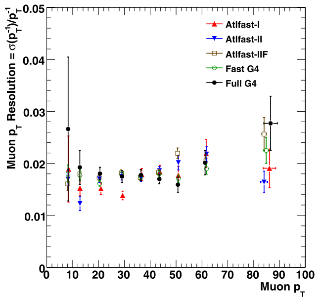
structed using only the muon spectrometer ( left ) and using both the inner detector and spectrometer ( right ). ATLFast-I only provides one type of muon, which is included in the right plot
