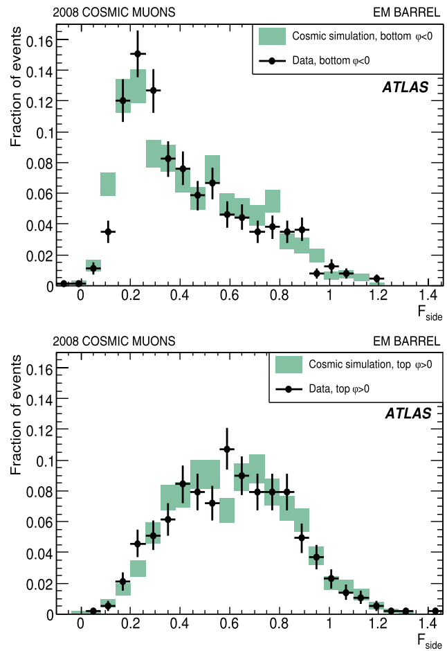
Fig. 23 Lateral shower containment in the first layer for “collision-like” (top panel) or “reverse” (bottom panel) electromagnetic showers for radiative cosmic muon data (dots) and Monte Carlo simulation (rectangles). The definition of the F_{\text{side}} is given in the text
