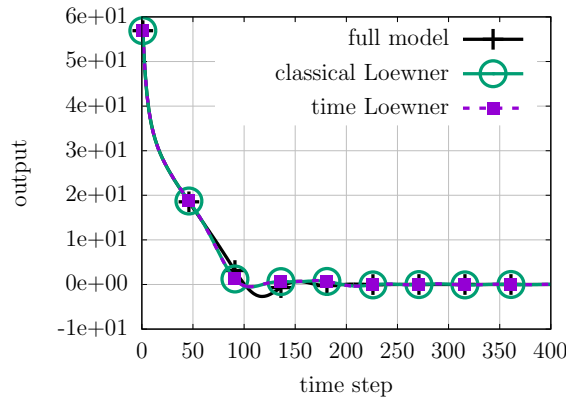
FIG. 5. Eady example: In this example, the time-domain output trajectory of the time-domain Loewner model has an approximation accuracy similar to that of the output trajectory of the classical Loewner model with respect to the full model.
