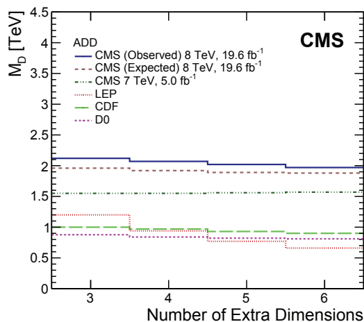
Figure 5: The 95% CL lower limits on the effective Planck scale, M_D , as a function of the number of extra dimensions in the ADD model, together with LO results from similar searches at the Tevatron [58, 59], LEP [60–63] and CMS [64].
