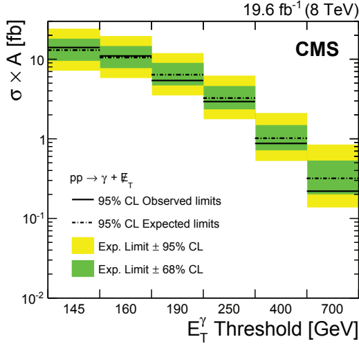
Figure 2: Upper limits at 95% confidence level (CL) on the product of cross section and acceptance as a function of the E_T^\gamma threshold ( >145 GeV) for the photon and E_T final state.
