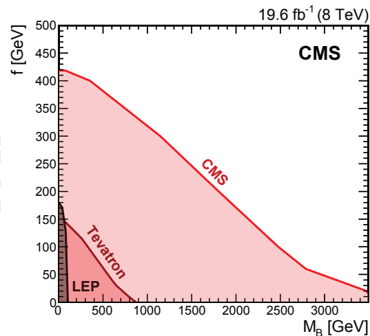
Figure 6: The 95% CL upper limits on the branon cross sections as a function of the branon mass M_B for N=1 . Also shown are the theoretical cross sections in the branon model for the brane tension scale f = 100, 200, 300 , and 400 GeV (top). Limits on f as a function of M_B , compared to results from similar searches at LEP [68] and the Tevatron [13] (bottom).
