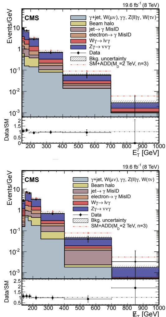
Figure 1: The photon E_T and \cancel{E}_T distributions for the candidate sample, compared with estimated contributions from SM backgrounds, and the predictions from the ADD model for M_D = 2 TeV and n = 3 . The horizontal bar on each data point indicates the width of the bin. The background uncertainty includes statistical and systematic components. The bottom panel shows the ratio of data and SM background predictions.
