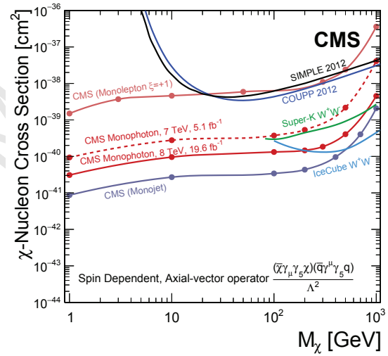
Figure 3: The 90% CL upper limits on the \chi -nucleon cross section as a function of the DM particle mass M_\chi for spin-independent couplings (top) and spin-dependent couplings (bottom). Results from the current search are shown as “CMS Monophoton, 8 TeV”. Shown are the limits from CMS using monojet [37] and monolepton [45] signatures (where \xi is the interference parameter addressing potentially different couplings to up- and down-type quarks and values of \xi = \pm 1 maximize the effects of interference). Also shown are the limits from several published direct detection experiments [46–55]. The solid and hatched yellow contours show the 68% and 95% CL contours respectively for a possible signal from CDMS [56]. Limits similar to those from the current search are obtained by ATLAS [57].
