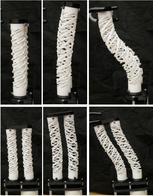
Fig. 3. Demonstration of a linear actuator created by a pair of handed shearing auxetic cylinders (HSA). Linear extension and compression is achieved just by the use of a single servo. Compliance is created due to the flexible nature of the PTFE tube that the HSA is patterned into.
