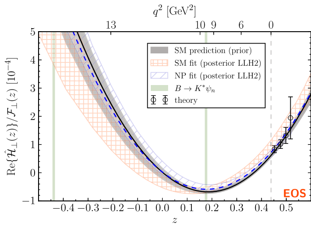
Fig. 1 Results of the prior and posterior fits for the ratio \text{Re}\{\hat{\mathcal{H}}_{\perp}(z)\}/\mathcal{F}_{\perp}(z) . See the text for details
