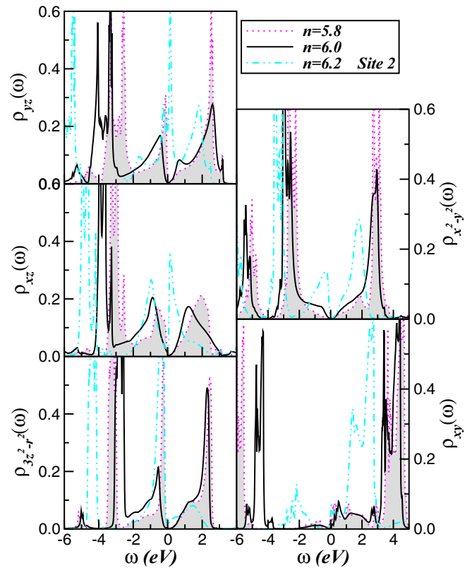
FIG. 5. Effect of electron/hole doping on the LDA+DMFT ( U = 5.0 eV, J_H = 0.7 eV) spectral functions for the Fe 3d orbitals of \text{Ca}_2\text{O}_3\text{Fe}_3\text{S}_2 at Site 2 . Notice the electron delocalization and the appearance of incoherent, pseudogapped shoulder quasiparticle resonances on different orbitals near the Fermi energy.
