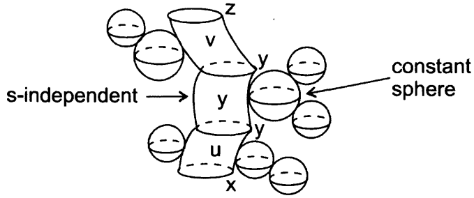
Figure 3-1: Picture of Floer trajectory (taken from Salamon [30])
