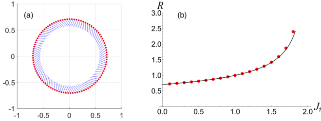
FIG. 1. (a) Scatter plot of a stable ring phase wave state in the (x, y) plane. The phase of each swarmalator is represented by a blue ray, and corresponds to the angle the ray makes with the positive x axis. As can be seen, in this state the spatial angle \phi_k = \tan^{-1}(y_k/x_k) of each swarmalator is correlated with its phase (i.e., \phi_k = \theta_k + \text{const} ). Parameter values were J_2 = 1 , J_1 = 0 , K = -0.003 , and N = 100 . (b) Radius of ring state versus J_1 . Red dots show simulation results for J_2 = 1 and N = 100 . The black curve shows theoretical prediction (7). To produce the data for the plot, we integrated the equations of motion (3) and (4) using Euler's method until the steady state was reached.
