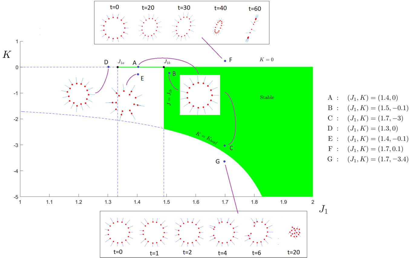
FIG. 2. Stability diagram for the ring phase wave state in (J_1, K) space with N = 15 , J_2 = 0 . Stable regions are indicated with a green color. Insets show the solution to Eqs. (3) and (4) corresponding to parameter values as shown (A through G) as scatter plots in the (x, y) plane. The phase of each swarmalator is represented by a blue ray, and corresponds to the angle the ray makes with the positive x axis. Initial conditions were taken to be a ring of radius 1, slightly perturbed. The ring is stable for parameter values A,B,C.
