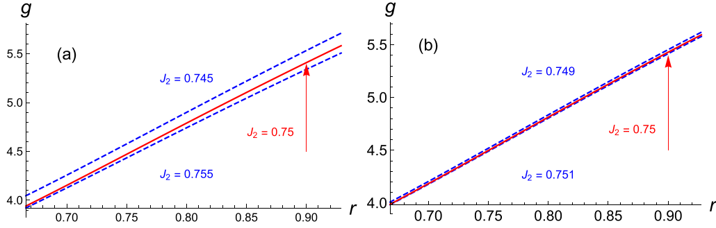
FIG. 6. Radial density g(r) for J_1 = 0.5 for values of J_2 in a neighborhood of 0.75. Blue dashed lines show are for J_2 \neq 3/4 calculated using expression (B18). The red solid line is for J_2 = 3/4 using expression (B22). The density g(r) varies smoothly as J_2 passes through 0.75. Panel (a) shows values J_2 = 0.745, 0.755 , which hug the curve at J_2 = 0.75 . In panel (b) we use a tighter neighborhood with extremal values 0.749, 0.751, which produces a tighter ‘hugging’. These results indicate that there is no change in the behavior of g(r) at the value J_2 = 0.75 .
