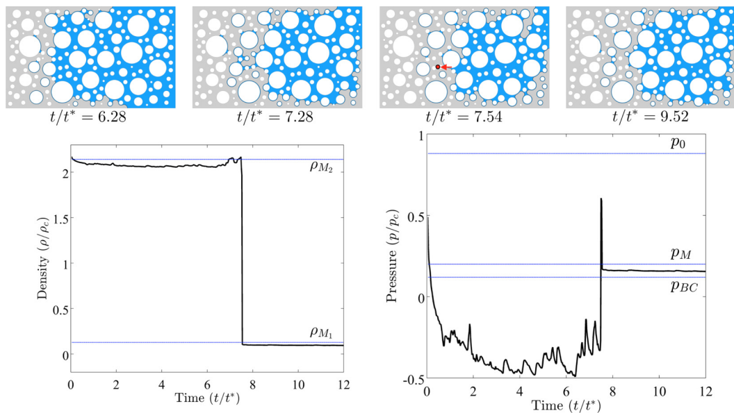
FIG. 22. Pressure and density fluctuations associated with the advancement of interfaces and the rupture of liquid films. We show the time evolution of density and pressure at a location at the surface of an obstacle (indicated with a red dot), together with snapshots of the density field immediately before and after the front has reached this location. The model parameters are \rho_{r0} = 2.2 , \rho_{rLB} = 0.07 , T_r = 0.7 , and \theta = 0^\circ . The Maxwell densities \rho_{M1} and \rho_{M2} , which are the thermodynamic equilibrium densities of vapor and liquid at this temperature, are indicated with dashed blue lines. The initial, left-boundary, and Maxwell pressures p_0 , p_{BC} , and p_M , respectively, are also indicated with dashed blue lines. In this case of drainage, pressures inside the vapor phase are significantly higher than in the liquid phase, which is consistent with a large capillary pressure.
