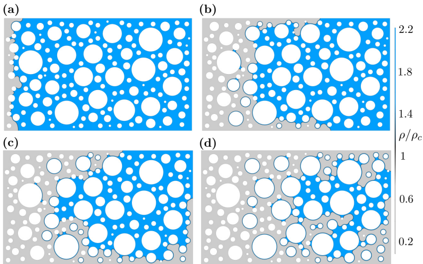
FIG. 15. Vaporizing front patterns are controlled by heterogeneity of the pore space. We show snapshots of a simulation with the same conditions as those of Fig. 13 ( \rho_r = 2.2 , \rho_{rLB} = 0.07 , T_r = 0.7 , and \theta = 0^\circ ) but with a distribution of obstacles that slightly promotes imbibition along the top and bottom boundaries. These patterns of vapor invasion resemble the invasion-percolation-like fronts in capillary fingering, as proposed in the context of drying [83,84].
