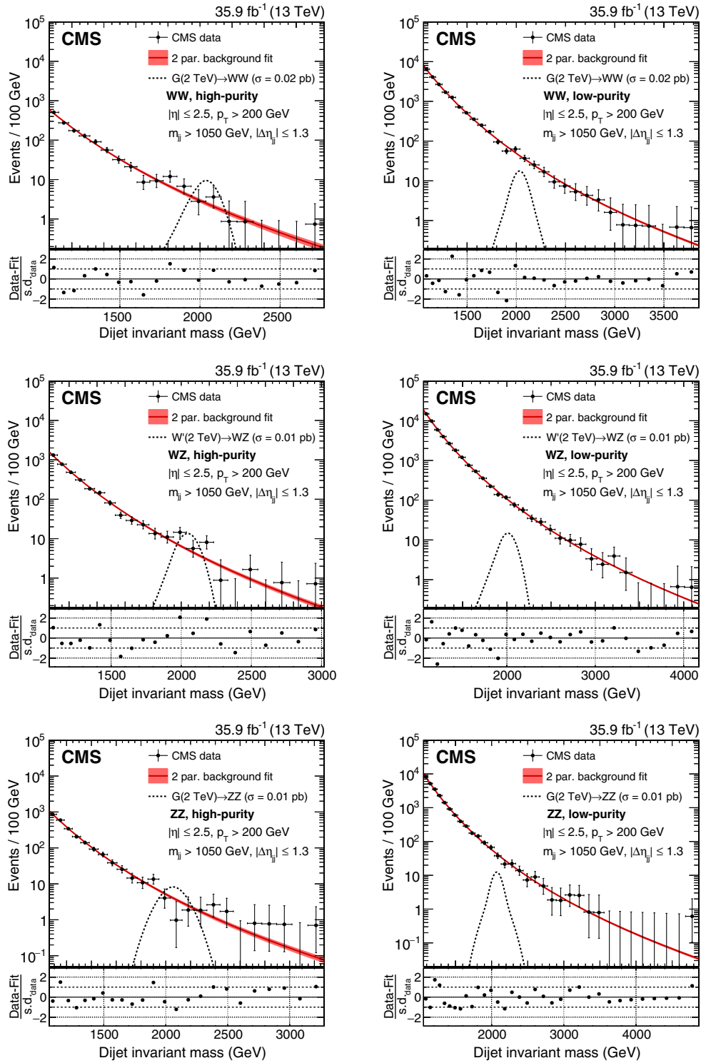
FIG. 4. The dijet invariant mass distribution m_{jj} in data. On the left, the HP, and on the right, the LP categories are shown for the WW , WZ , and ZZ categories, from upper to lower. The solid curve represents a background-only fit to the data distribution where the red shaded area corresponds to the one standard deviation statistical uncertainty of the fit. The dashed line shows the signal shape for a bulk graviton or W' of mass 2 TeV. The lower panels show the corresponding pull distributions, quantifying the agreement between a background-only fit and the data. Note that these fits do not represent the best fit hypotheses used in the statistical analysis where signal-plus-background fits are performed.
