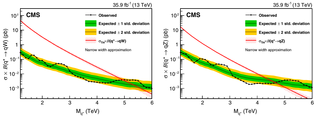
FIG. 8. Observed (black solid) and expected (black dashed) 95% C.L. upper limits on the production of an excited quark resonance decaying into qW (left) or qZ (right) as a function of resonance mass. Signal cross section uncertainties are displayed as red cross-hatched bands.
