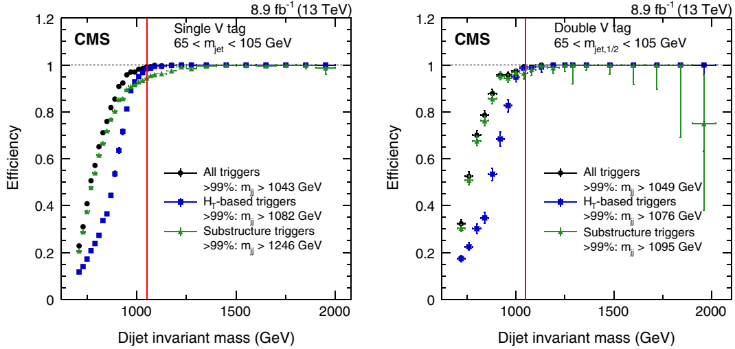
FIG. 1. Trigger efficiencies for jets passing the inclusive triggers (black), the H_T triggers (blue) or the substructure triggers only (green) as a function of dijet mass for the data-taking period with the highest trigger thresholds. Events are required to contain one jet with a soft-drop mass m_{\text{jet}} (left), or two jets with soft-drop masses m_{\text{jet},1} and m_{\text{jet},2} (right), within the signal window of the analysis. The vertical red line marks the selected threshold value.
