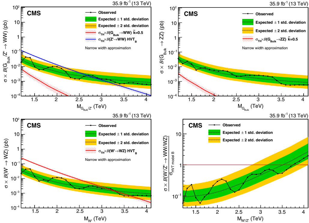
FIG. 6. Observed (black solid) and expected (black dashed) 95% C.L. upper limits on the production cross section of a narrow-width resonance decaying to a pair of vector bosons for different signal hypotheses. Limits are set (upper left plot) on a spin-1 neutral Z' and a spin-2 resonance decaying into WW , and compared with the prediction of the HVT model B (blue line) and a bulk graviton model with \tilde{k} = 0.5 (red line). Limits are also set in the context of a bulk graviton decaying into ZZ (upper right) with \tilde{k} = 0.5 and a spin-1 charged resonance decaying into WZ (lower left) and compared with the predictions of the models. Signal cross section uncertainties are displayed as cross-hatched bands. The plot on the lower right shows the 95% exclusion bounds on the signal strength for the triplet hypothesis of the HVT model B.
