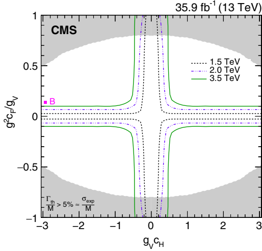
FIG. 7. Exclusion regions in the plane of the HVT model couplings for three resonance masses of 1.5, 2, and 3.5 TeV. The point B indicates the values of the coupling parameters used in the benchmark model. The regions of the plane excluded by this search lie outside of the boundaries indicated by the solid and dashed lines. The areas indicated by the solid shading correspond to regions where the theoretical width is larger than the experimental resolution of the present search and the narrow-resonance assumption is therefore not satisfied.
