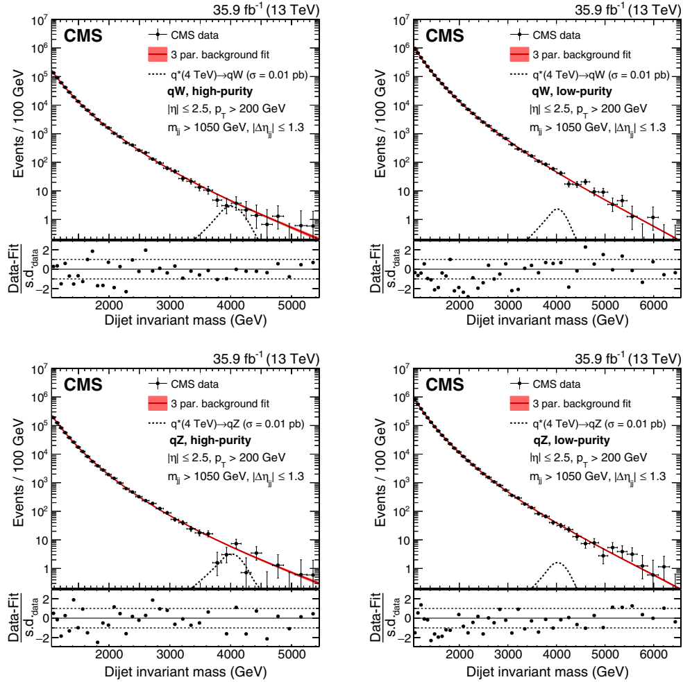
FIG. 5. The dijet invariant mass distribution m_{jj} in data. On the left, the HP, and on the right, the LP categories are shown for the qW and qZ categories, from upper to lower. The solid curve represents a background-only fit to the data distribution where the red shaded area corresponds to the one standard deviation statistical uncertainty of the fit. The dashed line shows the signal shape for a q^* with a mass of 4 TeV. The lower panels show the corresponding pull distributions, quantifying the agreement between a background-only fit and the data. Note that these fits do not represent the best-fit hypotheses used in the statistical analysis where signal-plus-background fits are performed.
