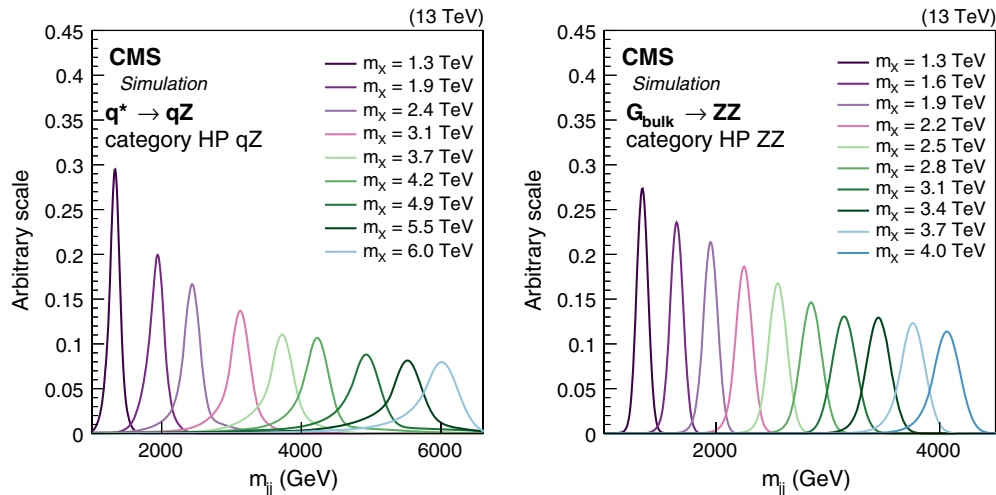
FIG. 3. Dijet invariant mass distribution for different signal mass hypotheses of the q^* \rightarrow qZ model (left) and the bulk graviton decaying to a pair of Z bosons (right) used to extract the signal shape in the HP category.
