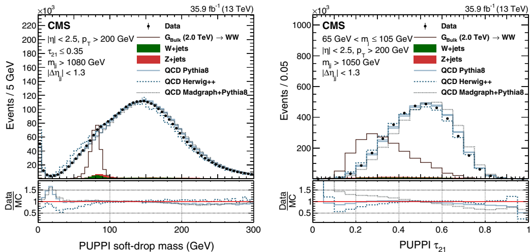
FIG. 2. The PUPPI soft-drop jet mass distribution (left) after preselecting and requiring \tau_{21} < 0.35 , and the PUPPI N-subjettiness \tau_{21} distribution (right) for data and simulated samples after preselection and requiring a soft-drop mass of 65 \leq m_{\text{jet}} \leq 105 GeV. The multijet production is shown for three different event generators. The W + jets and Z + jets events are stacked with the multijet sample generated with PYTHIA 8. For the PUPPI soft-drop jet mass distribution, the m_{\text{jj}} requirement has been raised from the analysis threshold of 1050 to 1080 GeV, since no requirements on the jet mass are applied. The lower subplots show the data over simulation ratio per bin.
