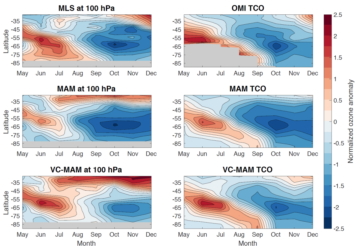
Figure 3. 2015 Normalized ozone anomalies from the 2004–2015 MLS, MAM, and VC-MAM time series shown as zonally averaged time-latitude maps (see text).
