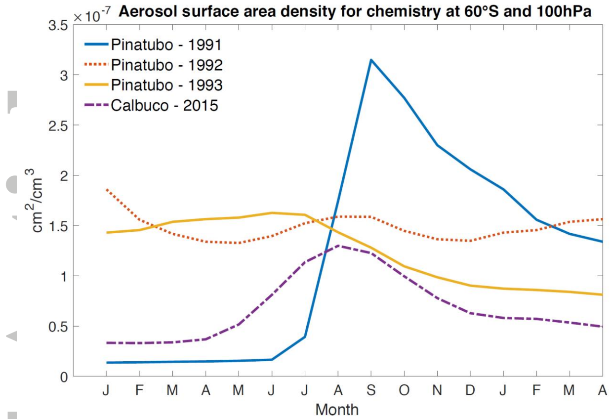
Figure 2. Aerosol surface area density for chemistry as derived by MAM at 60°S and 100 hPa for the Pinatubo 1991–1993 years and the Calbuco 2015 year.
