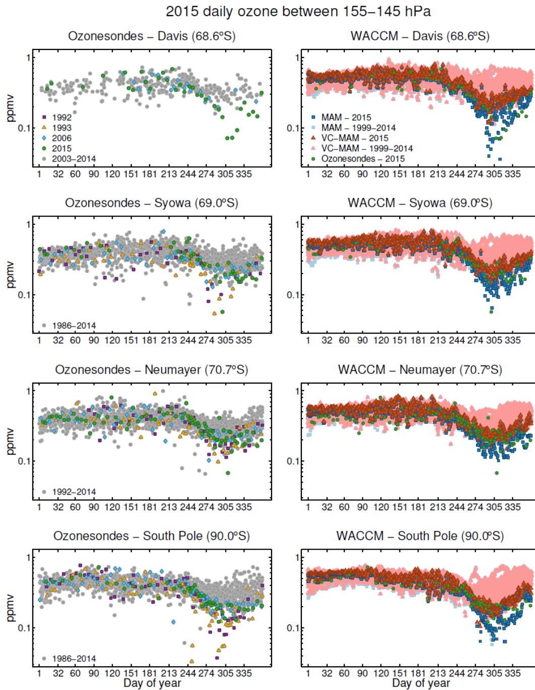
Figure 9. Ozonesonde data averaged between 155 and 145 hPa (left panels) and MAM and VC-MAM daily averaged values from their closest coincident model grid boxes at 150 hPa (right panels) plotted at their measured or simulated day of year. The ozonesonde measurements compare the large volcanically perturbed 1992 and 1993 Pinatubo years against 2015 and 2006, while the ozonesonde, MAM, and VC-MAM simulations are separately compared against each other for 2015.
