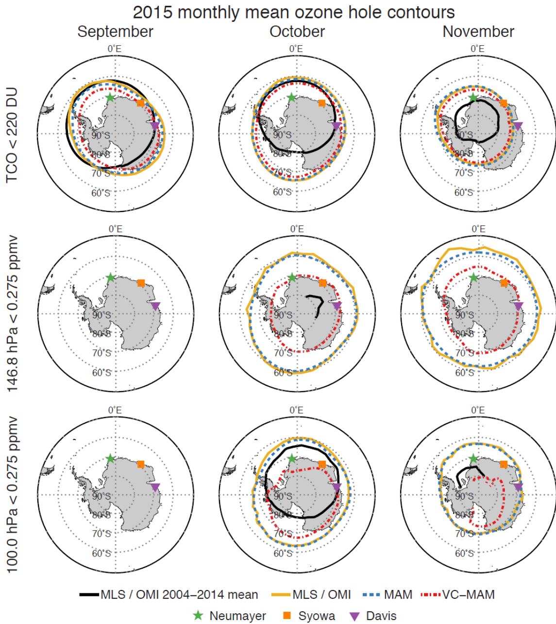
Figure 5. TCO 220 DU contour for OMI, MAM and VC-MAM and the .275 ppmv contour at 146.8 and 100 hPa for MLS, MAM and VC-MAM. The ozonesonde stations Neumayer, Syowa, and Davis are shown as symbols.
