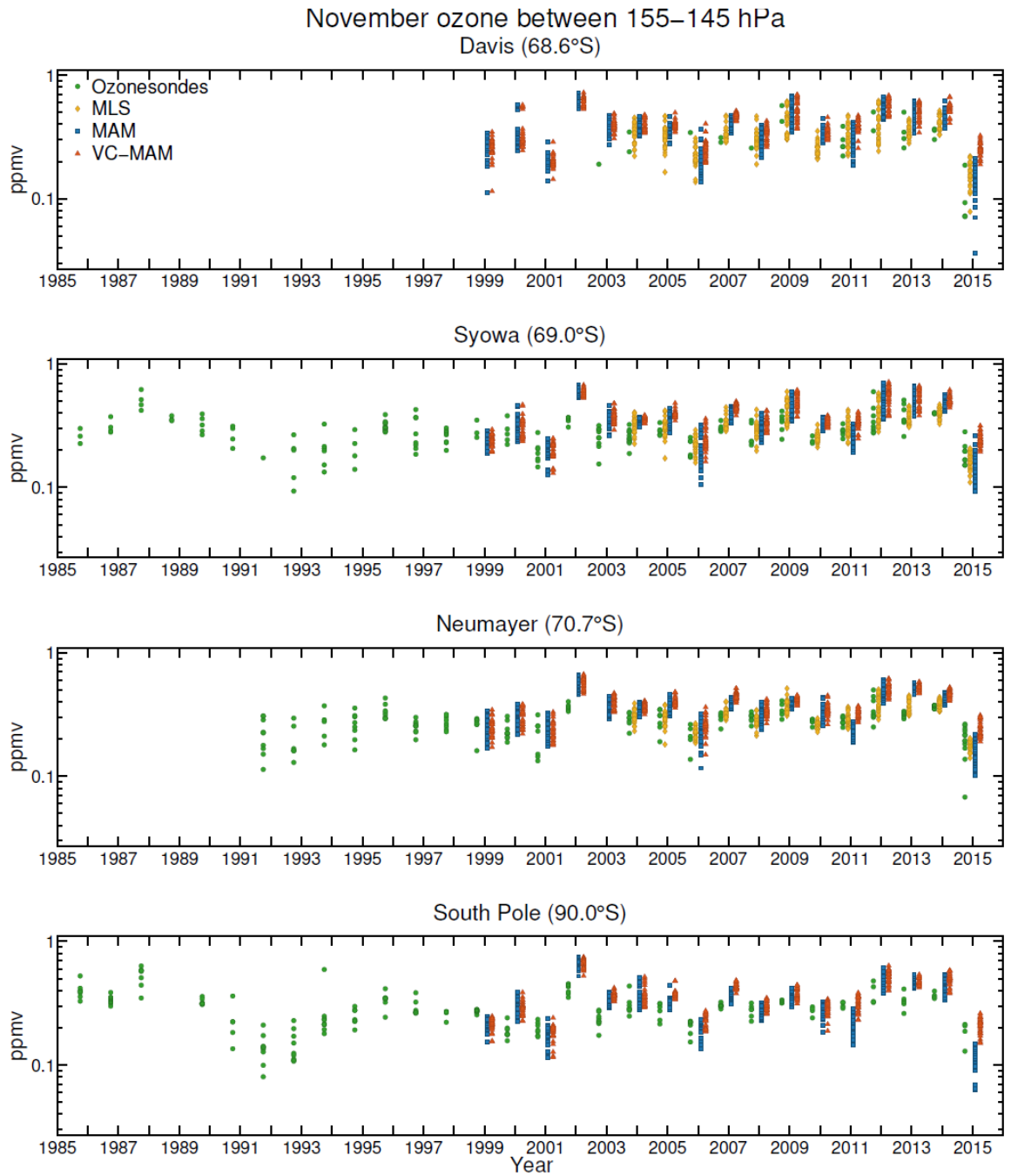
Figure 8. Same as Figure 7 for November.
