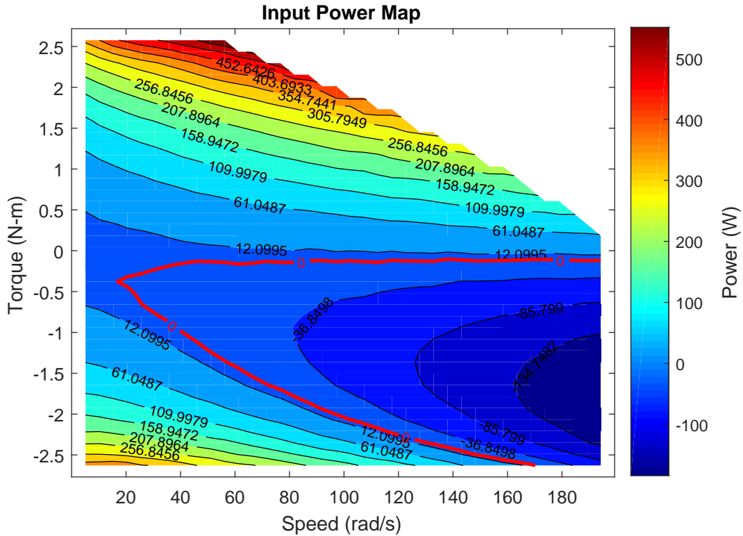
Figure 2-20: Input Power Map. The red contour indicates the zero-power operating points. Outside this region, the actuator sinks electrical power, and inside this region the actuator sources power.
