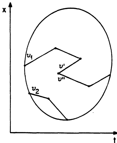
Figure 1: Random Polygonal Partition
