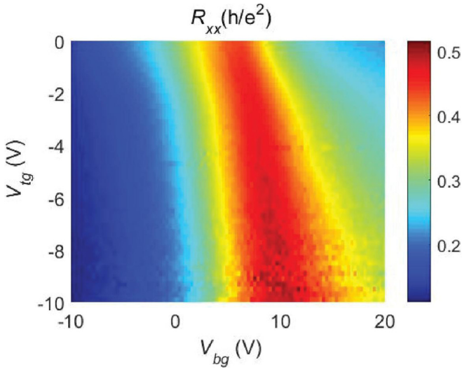
FIG. 11. Dependence of the longitudinal resistance R_{xx} on top- and back-gate voltages for device H 4 .
