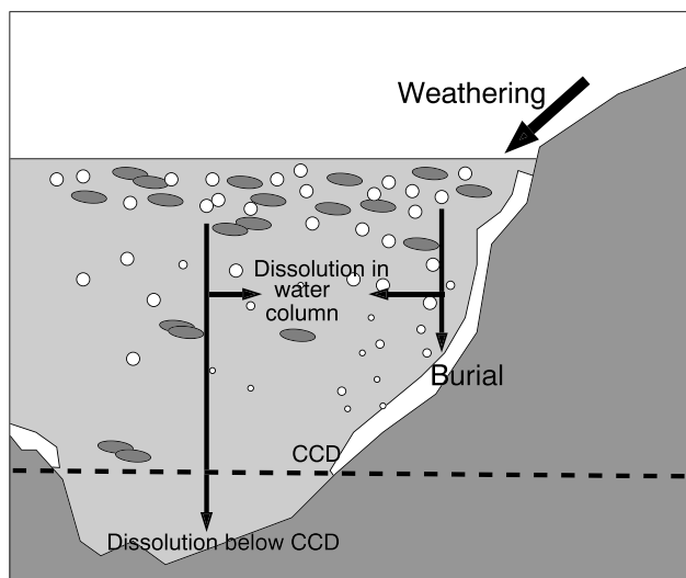
Figure 1. A schematic depiction of the input and output of alkalinity into and out of the ocean (figure adapted from Omta et al., 2013). Alkalinity is added to the ocean through river runoff and is consumed by calcifiers and removed from the ocean through calcifier sedimentation. Above the carbonate compensation depth (CCD), calcium carbonate accumulates, whereas it dissolves below the CCD. A decrease in deep-ocean [\text{CO}_3^{2-}] leads to a decrease in \text{CaCO}_3 output and, thus, an increase in deep-ocean [\text{CO}_3^{2-}] . This carbonate compensation feedback is thought to return the deep-ocean [\text{CO}_3^{2-}] to its equilibrium value on a multimillennial timescale.
