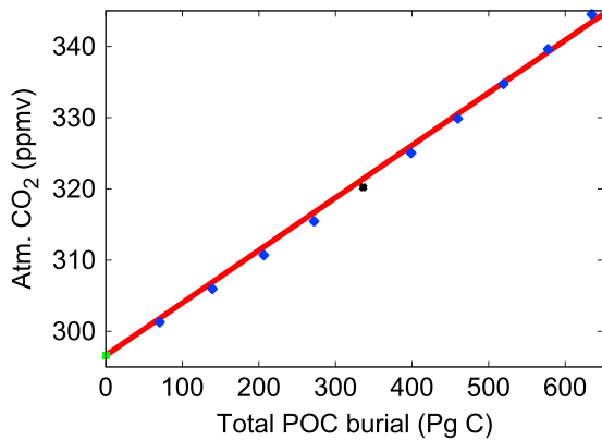
Figure 4. Atmospheric CO 2 as a function of the total amount of buried particulate organic carbon (POC), after a 250-kyr equilibration with carbonate compensation (blue diamonds). The green diamond indicates the spin-up simulation; the black cross stands for the simulation experiment shown in Figure 5. The red line indicates the slope predicted by relation (19), using M = 1.80 \times 10^{20} mol, X_{\text{CO}_2} = 300 ppmv, V = 1.40 \times 10^{18} m 3 , \gamma_A = 0.90 , C_{\text{sat}} = 2.00 mol/m 3 , B = 12.0 , and R_{\text{calc}} = 0.100 . In calculating this slope, the alkalinity change directly resulting from the remineralization of organic matter ( \delta A_{\text{reg}} = -R_{N:C} \delta C_{\text{reg}} ) was neglected, because this effect is not included in our multibox model.
