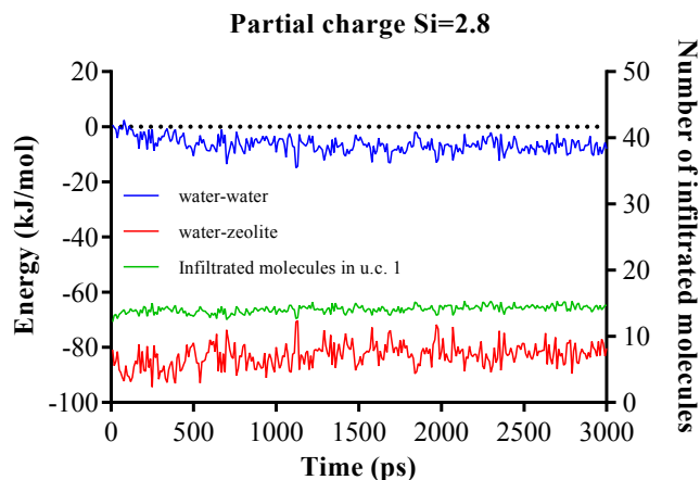
Figure 5: Attraction energy of infiltrated water in u.c.1 to water and zeolite for a high partial charge value. As the attraction to the zeolite is now greater, molecules are unable to freely infiltrate the zeolite pores.
