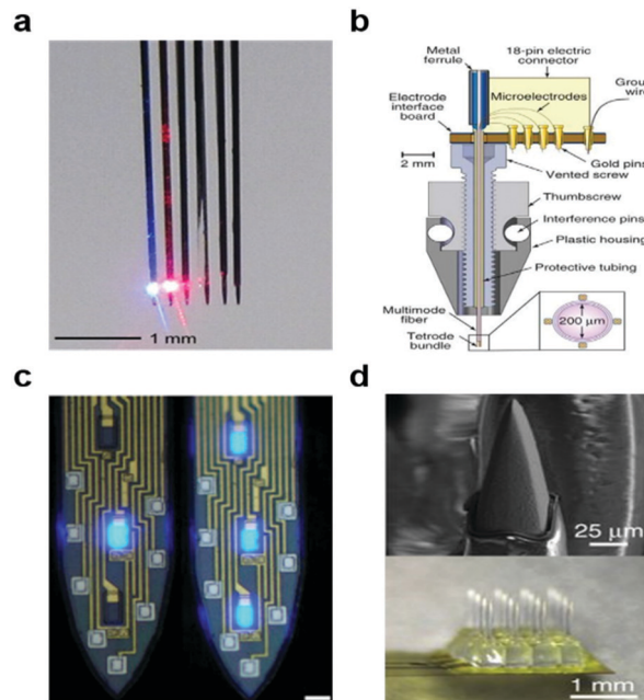
Fig. 9 Optoelectronic neural devices. (a) Multidiod arrays integrated with silicon multi-electrodes. Reproduced with permission from ref. 152. Copyright 2012 American Physiological Society. (b) Optrode with combination of ferrule and Ni/Cr based tetrode bundles. Reproduced with permission from ref. 158. Copyright 2012 Nature Publishing Group. (c) Monolithically integrated \mu\text{LED} on silicon neural probe. Reproduced with permission from ref. 164. Copyright 2015 Cell Press. (d) ZnO MOA device for multichannel intracortical neural recording and optical stimulation. Reproduced with permission from ref. 165. Copyright 2015 Nature Publishing Group.
