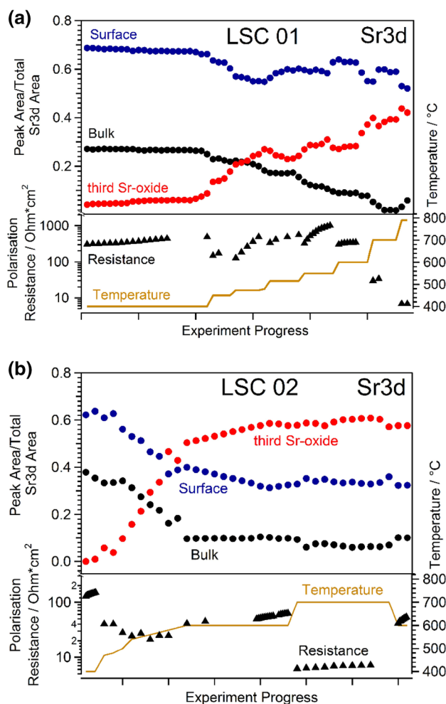
Fig. 6 Evolution of the three Sr 3d species as well as the electrode polarization resistance upon increasing temperature in 0.5 mbar O 2 . Plots (a) and (b) show results on two different samples with slightly different heating profiles. The top panel in each case shows the evolution of the relative intensity of Sr 3d XPS peak areas with increasing reaction temperature. The respective peak areas for the perovskite surface (blue) and bulk species (black) and the third Sr-oxide species (red) were obtained from the fitting of the Sr 3d peak as shown in Fig. 4. The bottom panel in each case depicts the evolution of the total polarisation resistance of the LSC electrodes obtained by impedance spectroscopy
