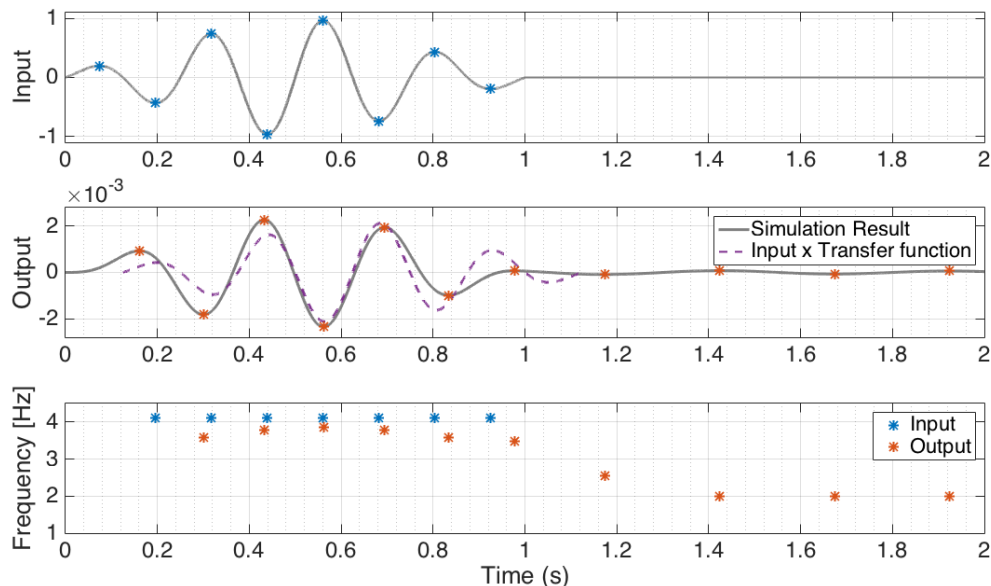
Figure 6. Modelled transient response of a simple pendulum to a sine-Gaussian injection. Simulink was used to model a simple pendulum with a resonance at 2 Hz. A one-second 4 Hz sine-Gaussian signal (top panel) was used as the input to show the response of the system (middle panel) compared with the input signal multiplied by the transfer function of the system at 4 Hz. Local maxima and minima of the time series can be used to calculate the frequency for each half-cycle (bottom panel). This simulation shows that even for this simple model, the transient response of the system deviates from the steady state frequency response at 4 Hz.
