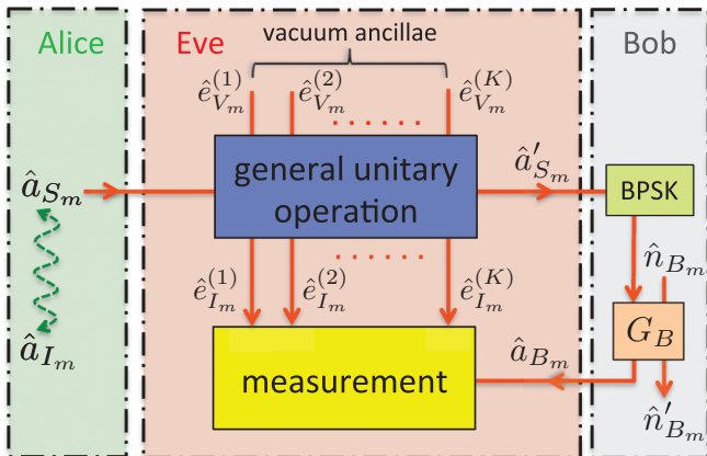
FIG. 5. Schematic of Eve's K -mode collective attack used to upper bound her Holevo information rate. BPSK: binary phase-shift keying. G_B amplifier gain. The dashed wavy line represents an entanglement that purifies the state of the \hat{a}_{S_m} mode.
