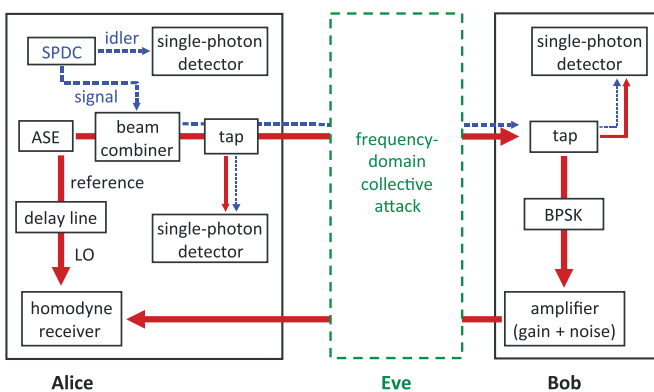
FIG. 1. Quantum channel setup for FL-QKD under frequency-domain collective attack. ASE: amplified spontaneous emission source. SPDC: spontaneous parametric downconverter. BPSK: binary phase-shift keying. LO: local oscillator.
