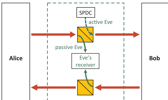
FIG. 2. Realization of Eve’s optimum frequency-domain collective attack. SPDC: spontaneous parametric downconverter. Eve’s SPDC signal beam (shown) is coupled to Bob through a beam splitter, while her SPDC idler beam (not shown) is retained for use in her receiver.
