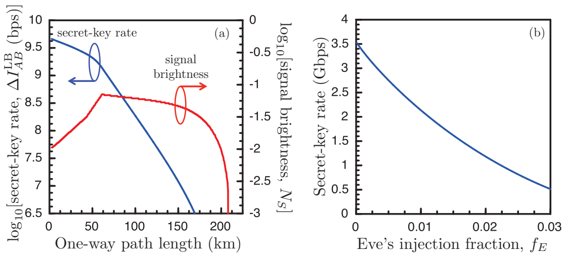
FIG. 3. (a) Lower bound on Alice and Bob's secret-key rate and Alice's optimum signal brightness when Eve mounts her optimum frequency-domain collective attack with injection fraction f_E = 0.01 . (b) Lower bound on Alice and Bob's secret-key rate vs f_E for a 50-km fiber link with all other parameters as in (a).
