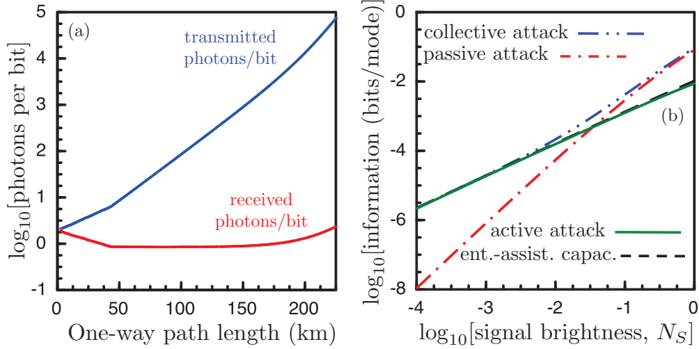
FIG. 4. (a) Alice’s transmitted photons per bit (ppb) and Bob’s received ppb when Eve mounts her optimum frequency-domain collective attack with injection fraction f_E = 0.01 . (b) Upper bounds on Eve’s optimum frequency-domain collective attack, passive attack, and active attack Holevo informations per mode—along with her entanglement-assisted capacity—as a function of Alice’s signal brightness, N_S , for a 50-km one-way path length assuming f_E = 0.01 .
