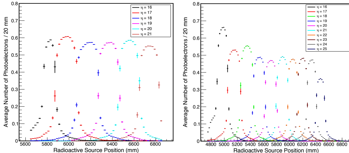
Figure 8. Response profiles for \phi = 5 layer 9 (left) and \phi = 6 layer 8 (right) sections.
