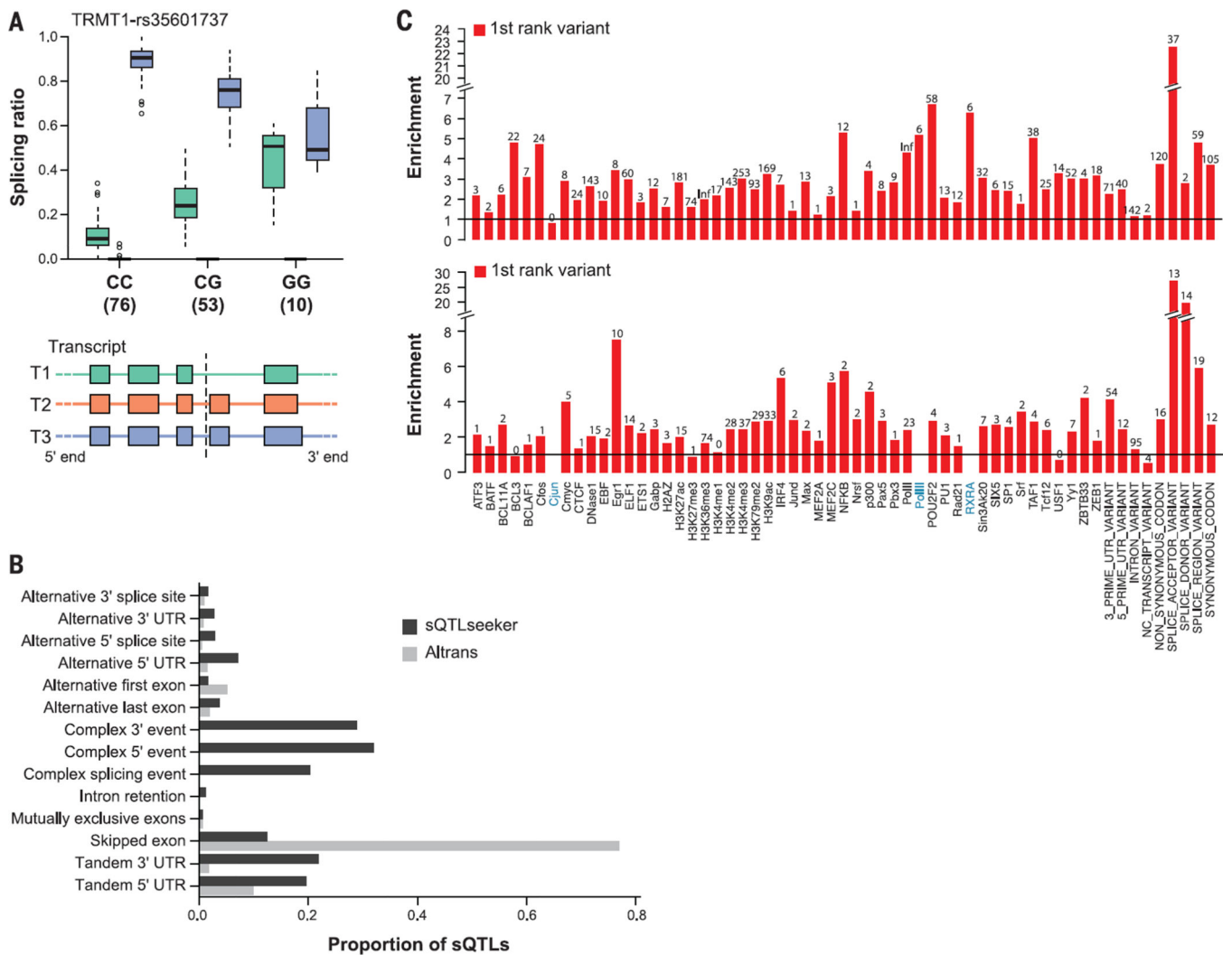
Fig. 5. Splicing QTLs
