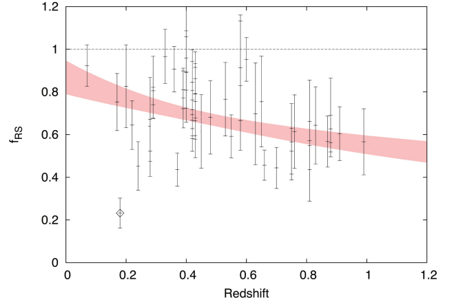
Figure 14. Red sequence fraction within the virial sphere of radius R_{200} as a function of redshift. The individual f_{RS} measurements are in black, and best fit trend is shown in pink. The typical RS fraction is 68 \pm 3\% at the pivot redshift z = 0.46 and mass M = 6 \times 10^{14} M_{\odot} with intrinsic variation at the 14% level. The best fit redshift trend f_{RS} \propto (1+z)^{-0.65 \pm 0.21} has characteristic values around 55% at z = 1 and 80% at z = 0.1 . One LMC cluster appears marked with an open diamond.
