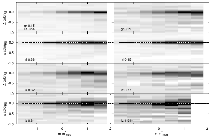
Figure 6. Stacked cluster galaxy color–magnitude distributions (left) for the 8 different redshift bins (see Table 2). The magnitude scale is defined relative to the m_*(z) of our passive evolution model, and the color offset is defined with respect to our tilted RS model (see Section 3.1.1). A common grey scale across all bins represents the completeness corrected and background subtracted number density of galaxies per magnitude and color bin. The RS is clearly apparent at all redshifts, extending cleanly to m_* + 2 in the lower redshift bins. On the right is the stacked galaxy color distribution for the same redshift bins. All distributions are normalized to unit area. At higher redshift the distribution of galaxies bluer than the RS grows more prominent, and the RS has lower contrast.
