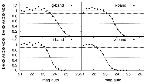
Figure 2. Completeness functions in each band for SPT-CL J0423-6143. We compare the object counts observed toward the cluster to the counts from deeper data from the COSMOS survey. The resulting completeness curve is fit by an error function, which we use to estimate 50% and 90% completeness.
