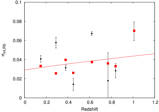
Figure 8. Black points mark the color measurement-noise corrected widths of the RS at each redshift using the band combinations in Table 2. The red points are the estimated RS widths in the rest frame g-r color, given the width in the observed band combination. There is no compelling evidence for RS width evolution within the rest frame bands (see Equation 8).
