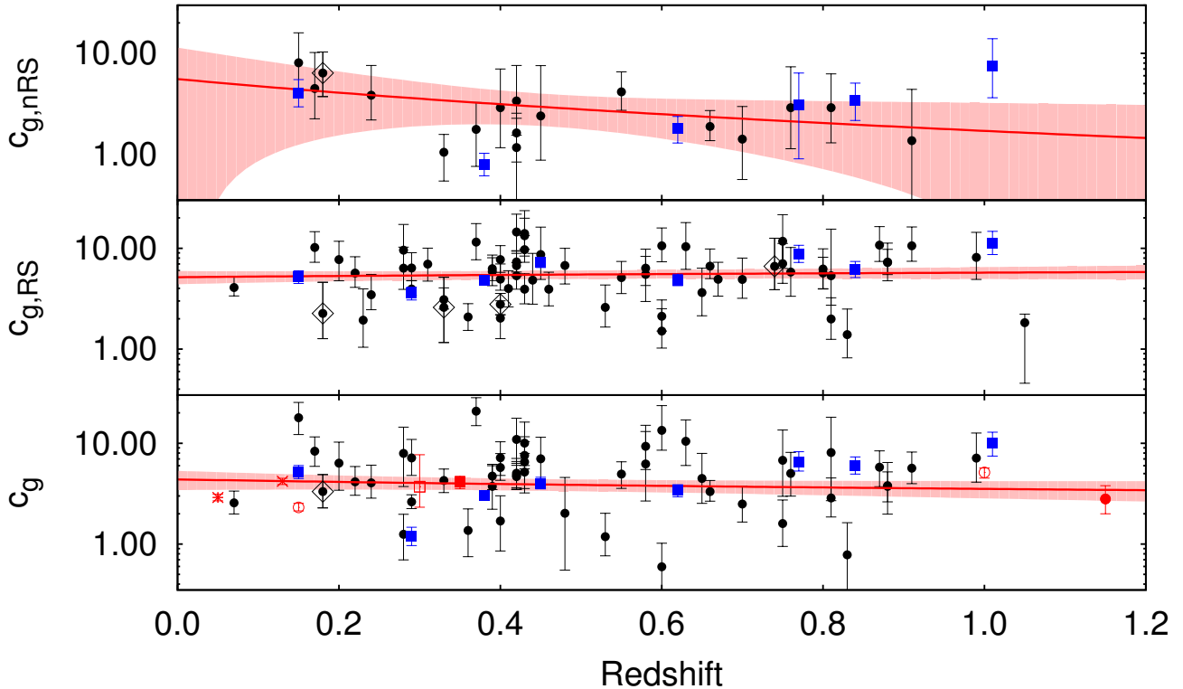
Figure 12. Redshift trend of the concentration parameter for the non-RS blue (top), RS (middle) and full (bottom) populations. The black points (blue) show the best fit NFW concentration for individual clusters (stacks). The line marks the best fit redshift trend and 1\sigma region (see Table 4). The characteristic concentrations for the non-RS, RS and full populations are 1.59 \pm 0.53 , 5.47 \pm 0.53 and 3.89 \pm 0.52 , respectively. There are no statistically significant mass or redshift trends. Considerable cluster to cluster scatter at the 55% to 38% level is apparent. The red points show various published results that are described in the text (Section 4.2.3). In addition, we mark the clusters close to the Large Magellanic Cloud ( \delta < -63^\circ ) as black open diamonds.
