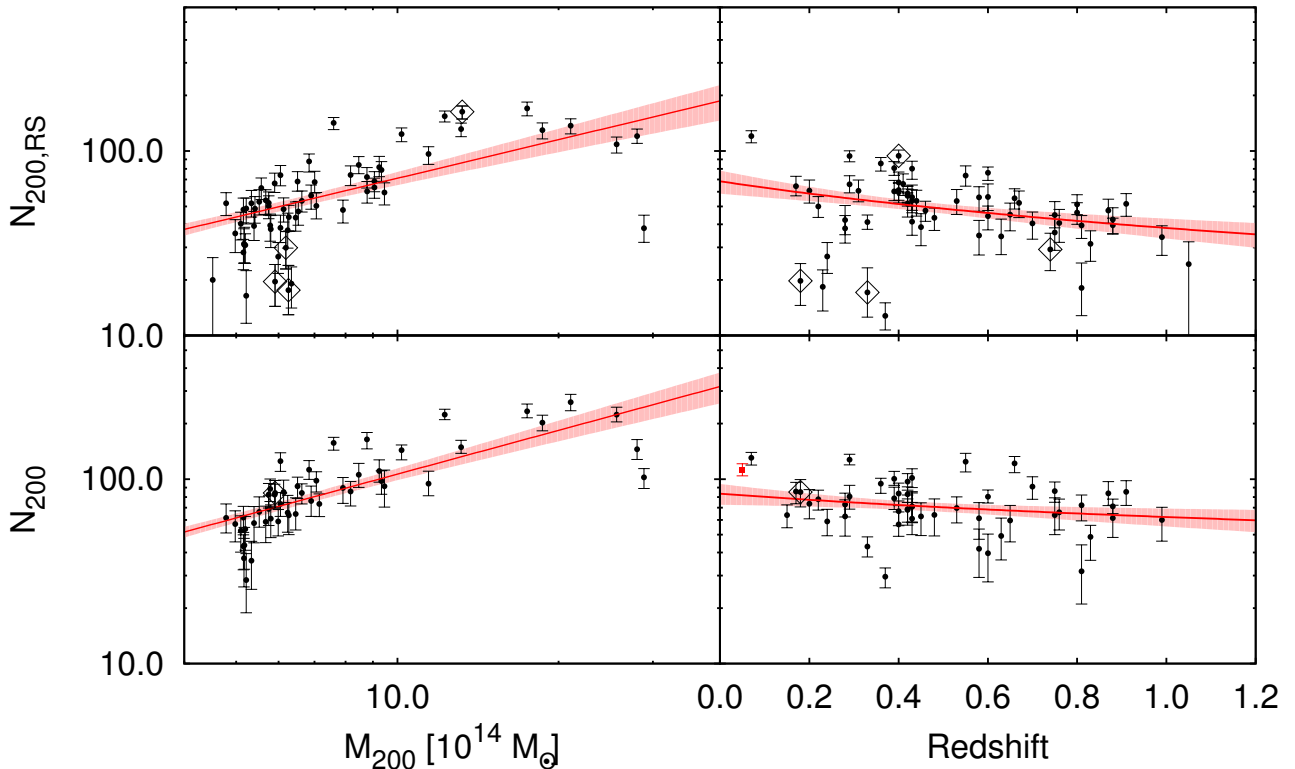
Figure 13. The HON from measurements of N_{200} from the galaxy radial profiles is plotted versus mass (left panels), and the HON normalized to a mass of 6 \times 10^{14} M_{\odot} is plotted versus redshift (right panels). In both cases the full (RS) population appears on bottom (top), and both populations have N_g \propto M^B where B < 1 (see Table 4). We find no clear evidence of a redshift trend in the full population, but the RS population shows a 2.5\sigma trend for falling HON with redshift. The 1\sigma region (Equation 14) for each fit is plotted in red. The clusters near the LMC ( \delta < -63^\circ ) are more contaminated by stars and are marked with black open diamonds.
