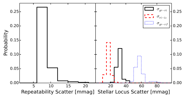
Figure 1. Distribution of single epoch photometric repeatability scatter (left) for multiple measurements of the same stars in our ensemble of 74 clusters. The bands griz have a median scatter of 7.6, 7.6, 7.7 and 8.3 mmag, respectively. The distribution of orthogonal scatter about the stellar locus is shown on the right for three color-color spaces. The scatter distributions for these three spaces have a median scatter of 17, 32 and 57 mmag.
