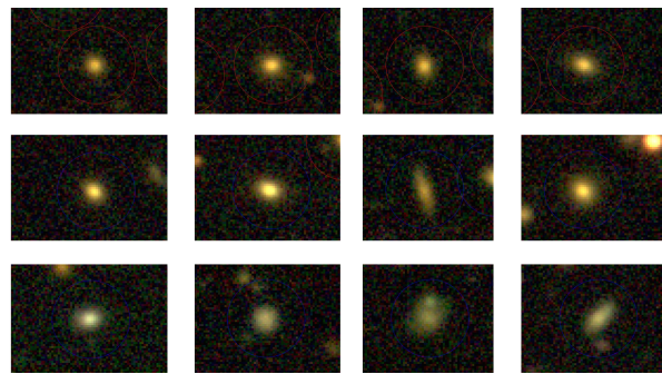
Figure 7. Image gallery of galaxies at R < R_{200} within the field of SPT-CL J2351-5452. The top row contains 4 examples of galaxies with a high likelihood ( \geq 90\% ) of being RS members, and the second row shows galaxies with intermediate likelihood ( \sim 40\% ). We note that these constitute a population of galaxies whose colors lie between those of the RS and the bluer spirals. The third row contains galaxies with a low likelihood ( \leq 20\% ) of being RS members. The majority of these are bluer disk galaxies.
