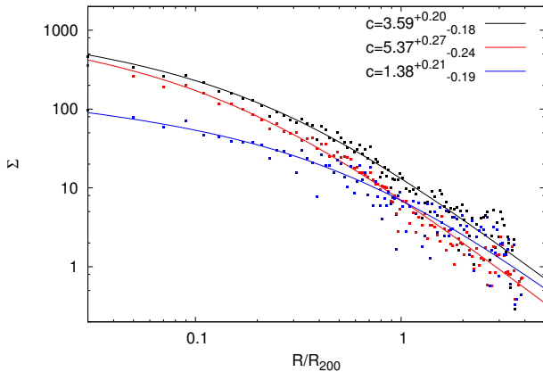
Figure 10. The black, red and blue points (and lines) show the stacked, background subtracted radial profiles and their best fit NFW models for the full, RS and blue non-RS populations, respectively. We show the quantity \Sigma = N/(A_{200}) , where A_{200} is the projected virial area. These stacks contain all clusters in the sample except for SPT-CL J0330-5228, which has no i-band coverage. All individual profiles extend to 4R_{200} . The RS and blue non-RS populations are selected using the observed color distributions in eight redshift bins (see Equation 5). The RS population is strongly clustered, whereas the blue non-RS population is clustered but with a lower concentration.
