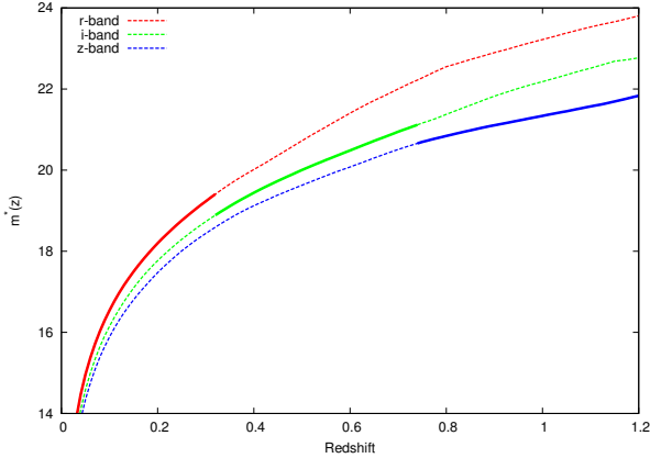
Figure 3. The characteristic magnitudes m_*(z) from the CSP model that are used for this study. In a companion paper we use measurements of m_* for this cluster sample to test and calibrate this model, finding it to be an excellent description of the cluster galaxy population characteristic magnitude and its evolution with redshift. The bands are color coded and the solid lines mark the redshift ranges where each band, redward of the 4000 Å break, is used.
