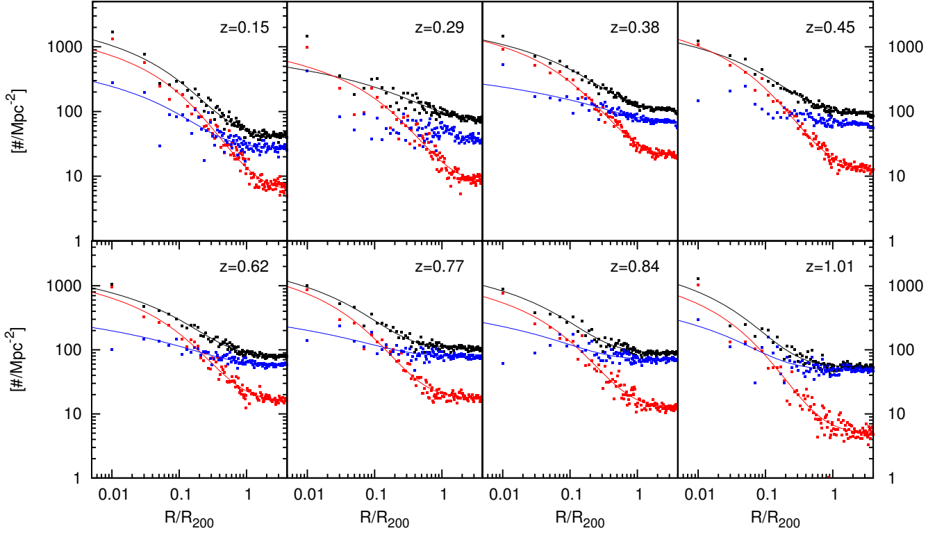
Figure 11. The color coding is the same as in Figure 10, but here the stacks without background subtraction are shown for the eight different redshift bins. Again, all profiles extend to 4R_{200} . In each redshift bin we find that the blue non-RS population is concentrated toward the cluster center but with lower concentration than the RS population. The concentrations from the stacks show no statistically significant mass or redshift trends (see Table 4). No model is shown for the blue non-RS population in redshift bins 2 and 4, because the concentration is not constrained.
