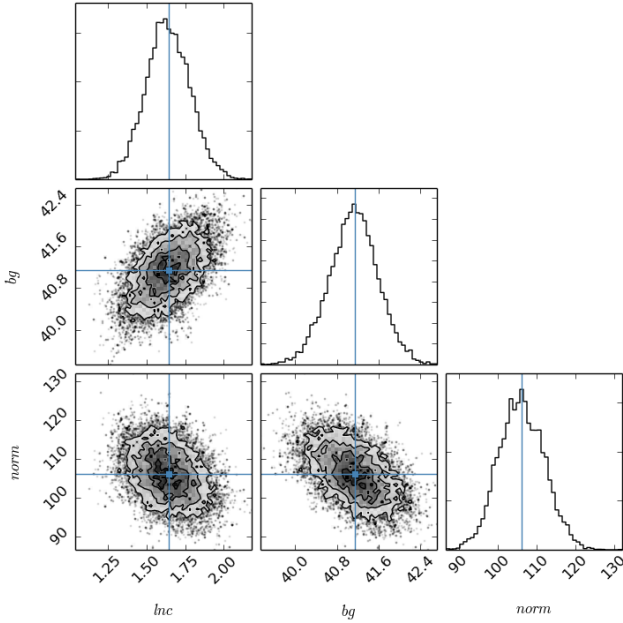
Figure 9. Parameter constraints for the stacked cluster profile using the full population within the redshift range 0.07 < z < 0.23 . We show the joint and fully marginalized constraints in \ln(c) , the background bg and the number of galaxies norm projected within R_{200} . The best fit is marked with the vertical blue lines.
