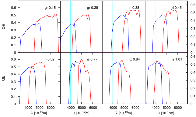
Figure 5. Plots of the average relative throughput or quantum efficiency (QE) in the rest frame of the blue and red bands we use within the 8 different redshift bins defined in Table 2. Redshifts and observed band combinations are noted in each panel, and 4000 Å is marked in cyan. By adopting different band combinations as a function of redshift we are able to probe similar portions of the rest frame SED over the full redshift range.
