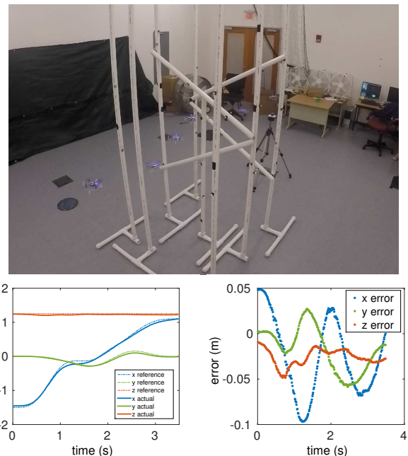
Fig. 5: Top is a composite picture of the quadrotor executing the planned trajectory through the environment containing 11 poles. Bottom left shows the tracking of position over time and bottom right the corresponding error.
