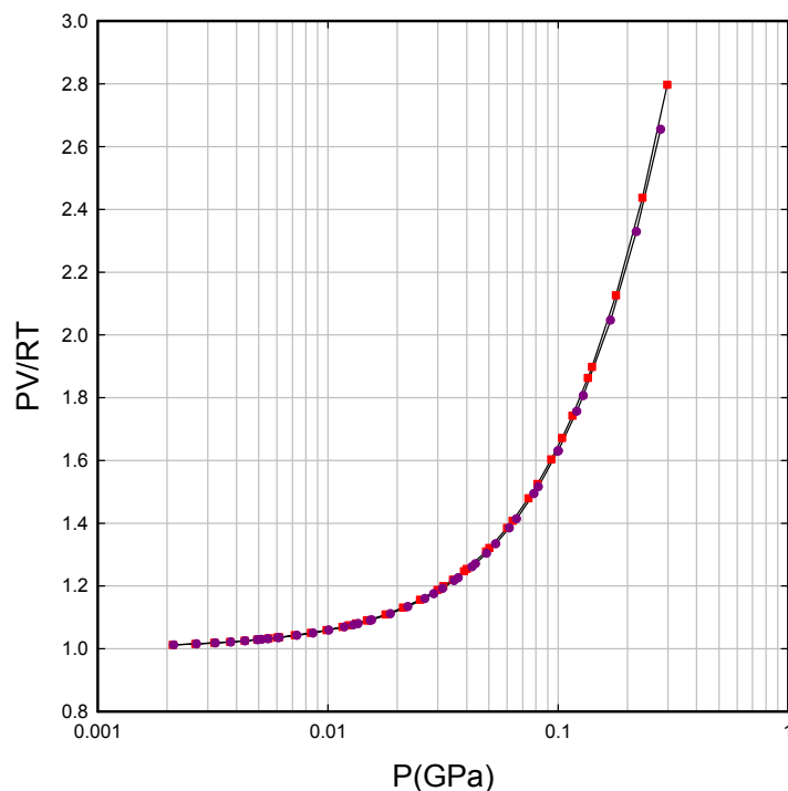
Figure 6. Compression ratio PV/RT for H_2 (light red squares) and for D_2 (dark pink circles) at 25^\circ C as a function of pressure.
