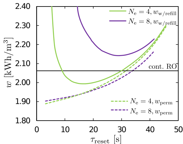
Figure 13: The effect of energy consumption for cycle reset on overall w and the potential for energy savings with batch RO for the case of batch RO with 4 and 8 elements.
