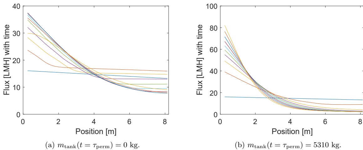
Figure C.17: Flux profile within the membrane module plotted at equal time intervals over the cycle time of the batch process. Note that the range of flux values is higher for the case with a larger external tank.
