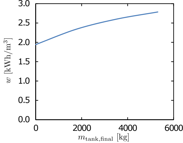
Figure 3: Specific energy consumption as a function of external brine tank mass at the end of the permeate producing portion of the cycle time, t = \tau_{\text{perm}} (Other parameters are fixed at their baseline values listed in Table 1). m_{\text{tank,final}} must be close to zero to ensure w is lower than that of continuous RO.
