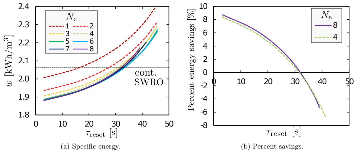
Figure 11: Effect of cycle reset time on energy savings with batch operation. Note that this plot does not account for the energy required by the refill pump, which is included in the next subsection.
