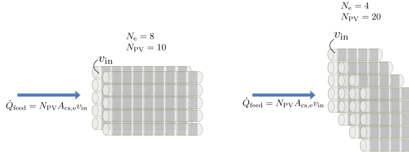
Figure 7: The number of membrane elements in series or the length of the membrane elements can be changed in batch RO without changing flux or RR. While doing so, the number of pressure vessels and length of each PV can also be modified. The overall feed volume flow rate and hence the size of the pumps may have to be adjusted when changing N_{\text{e}} .
