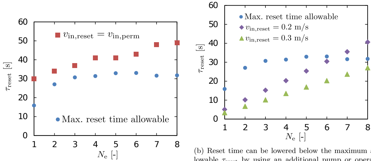
(a) Default reset time with existing pumps is higher than the maximum allowable reset time for energy savings, which is obtained from Fig. 11a
