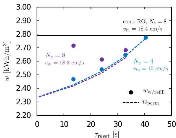
Figure D.18: Comparison of batch operation and single-stage RO at a higher recovery of 63.5% and overall flux of 18.85 LMH.
