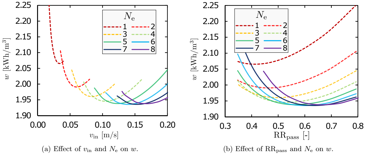
Figure 9: Effect of varying the number of elements and inlet feed velocity on specific energy consumption.
