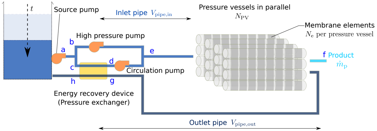
Figure 1: Schematic representation of batch RO with an atmospheric pressure feed tank. The impact of feed volume in the tank at the end of the operating cycle and volumes of the inlet and outlet pipes ( V_{\text{pipe,in}} , V_{\text{pipe,out}} ) relative to the feed volume inside the membrane elements is studied. Thereafter, the effect of N_e , N_{PV} and feed inlet velocity ( v_{\text{in}} ) are studied. The setup required for the cycle reset process is depicted in Fig. A.15.
