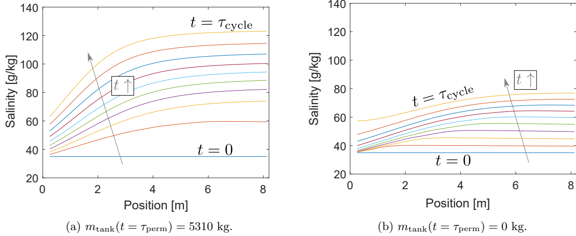
Figure 4: Feed salinity profile within the feed channel plotted at equal time intervals over the permeate producing time of the batch process.
