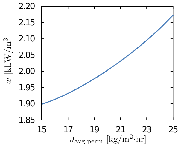
Figure 10: Increasing J_{\text{avg,perm}} is one method of compensating for the change-over or reset time between batch cycles, but this is accompanied by an increase in w .
