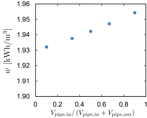
Figure 6: Effect of fraction of pipe volume in the inlet. Having a larger fraction of the total pipe volume in the outlet pipes results in a lower energy consumption.
