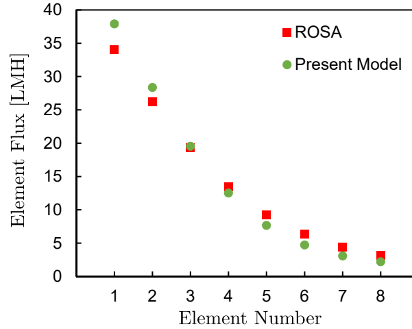
Figure B.16: Comparing model element flux with ROSA predictions.
