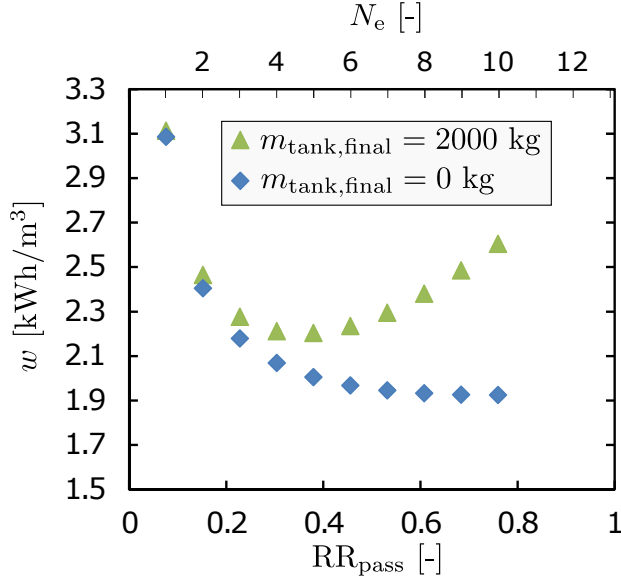
Figure 8: Effect of RR_{\text{pass}} at two external tank sizes. RR_{\text{pass}} is modified by changing N_e from 1 to 10. There exists an optimal intermediate value of per-pass recovery ratio only for the case of large external tank.
