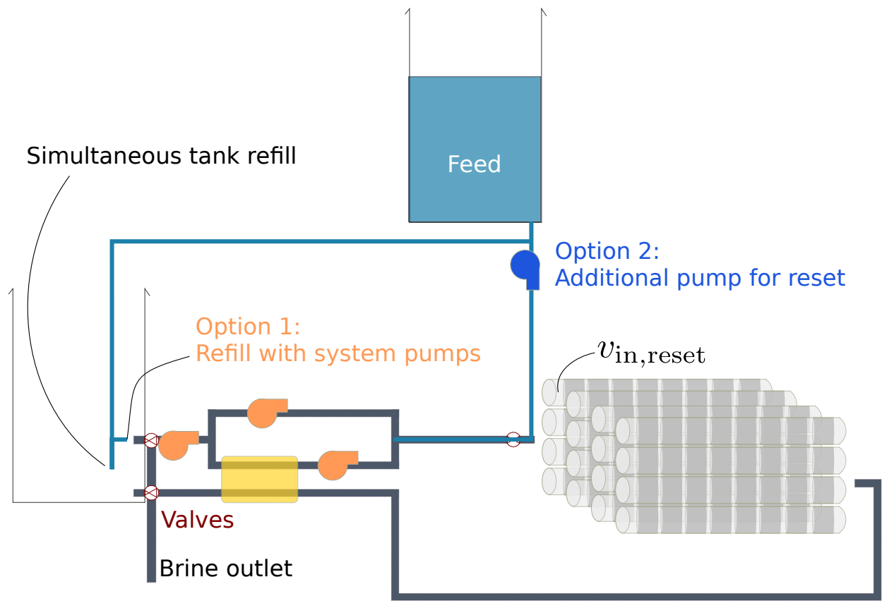
Figure A.15: System refill design.
