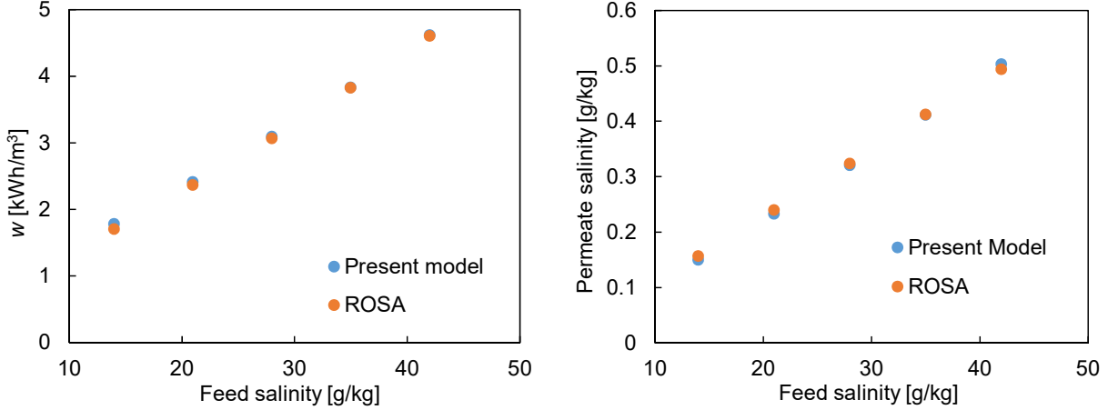
(a) Specific energy consumption (no ERD).
