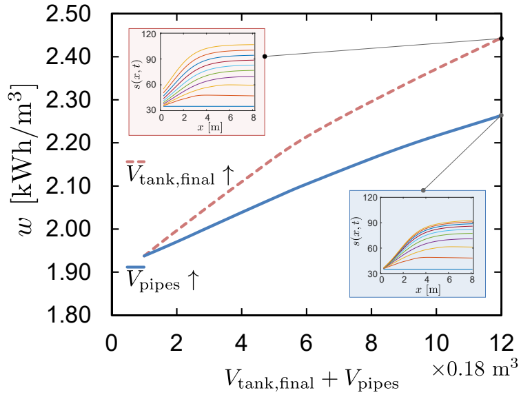
Figure 5: Effect of increasing the volume of pipes at fixed V_{\text{tank,final}} = 0 . The impact of increasing V_{\text{tank,final}} at fixed V_{\text{pipes}} = 0.18 \text{ m}^3 (which is the baseline volume of pipes considered in this study) is also reproduced for comparison. Insets show the salinity profiles within the membrane elements over time for the two cases, to explain the lower w when increasing V_{\text{pipes}} as opposed to V_{\text{tank,final}} .
