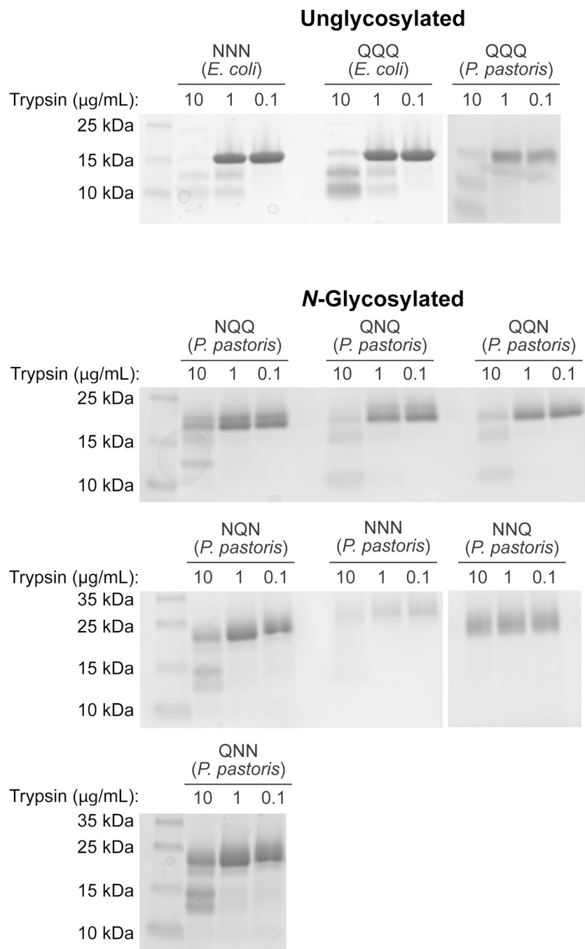
Figure 5. SDS-PAGE gels showing the effect of trypsin on RNase 1 glycoforms. An RNase 1 glycoform (1 mg/mL) was incubated with trypsin (0.1, 1, or 10 \mu\text{g/mL} ) at 37 °C for 1 h. The trypsin was inactivated with PMSF, and the products were subjected to electrophoresis in a 15% w/v gel and visualized by staining with Coomassie blue.
