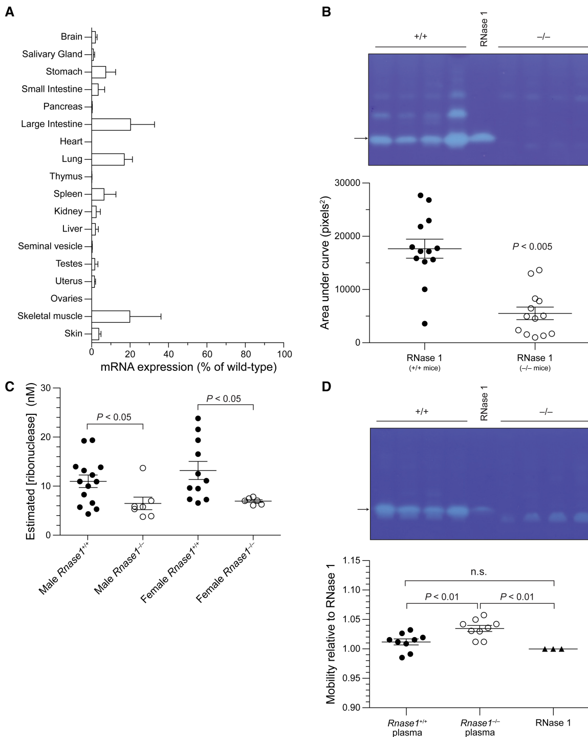
FIGURE 2. Verification of the loss of RNase 1 in Rnase1 -/- mice. (A) Bar graph showing the tissue-specific expression of Rnase1 in Rnase1 -/- mice relative to that in Rnase1 +/+ littermates as measured by qPCR. Mice were matched for sex. n = 3 per tissue. Data were normalized to the geometric mean of three reference genes. (B) Zymogram of plasma samples (0.5 \mu L) from Rnase1 +/+ or Rnase1 -/- mice used to evaluate ribonucleolytic activity relative to recombinant murine RNase 1 (100 pmol; arrow). Graph showing total ribonucleolytic activity, which was quantified by integration of a densitometry map of each lane and found to be significantly lower in Rnase1 -/- mice than in Rnase1 +/+ mice. (C) Graph showing plasma ribonuclease concentration by genotype and sex as estimated from ribonucleolytic activity. Concentration was calculated with Equation 1 and k_{cat}/K_M = 8.6 \times 10^6 \text{ M}^{-1} \text{ sec}^{-1} . n \geq 6. (D) Zymogram of plasma samples (0.5 \mu L) treated with PNGase F and of recombinant murine RNase 1 (100 pmol; arrow). The mobility was measured from the position of the well, and normalized to the mobility of recombinant murine RNase 1 (center lane). The position of the primary band present in Rnase1 -/- plasma differs from that in wild-type plasma (arrow).
