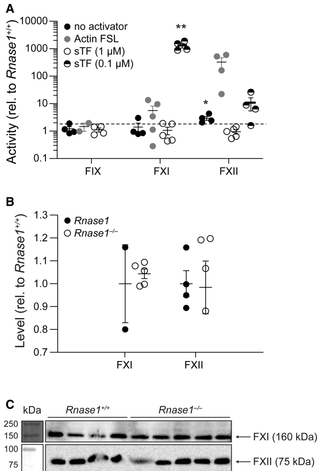
FIGURE 6. Effect of Rnase1 on the levels of FXII and FXI. (A) Graph showing the activity of FIX, FXI, and FXII in the plasma of Rnase1 -/- relative to that in Rnase1 +/+ mice. n \geq 3 . (B) Graph showing the level of FXI and FXII in the plasma of Rnase1 -/- and Rnase1 +/+ mice, normalized to the average expression in Rnase1 +/+ mice. n \geq 3 . (C) Representative immunoblots to probe for FXI and FXII. Molecular weight markers are indicated from separate exposures. (*) P < 0.05 ; (**) P < 0.001 .
