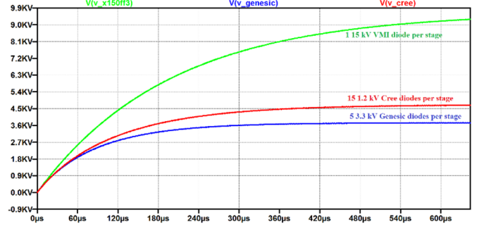
Fig. 4 Output voltages of three single-stage full-wave cockroaft-walton multipliers using three different diodes
