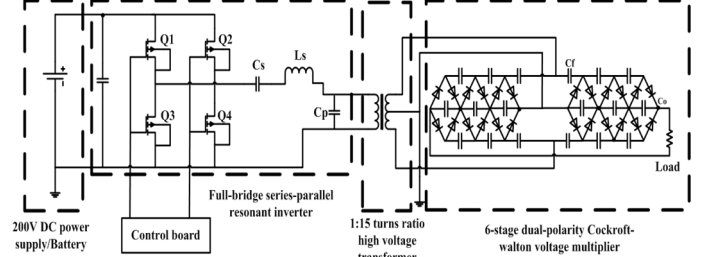
Fig. 5 Topology of a 40 kV 750 W dc-dc converter
