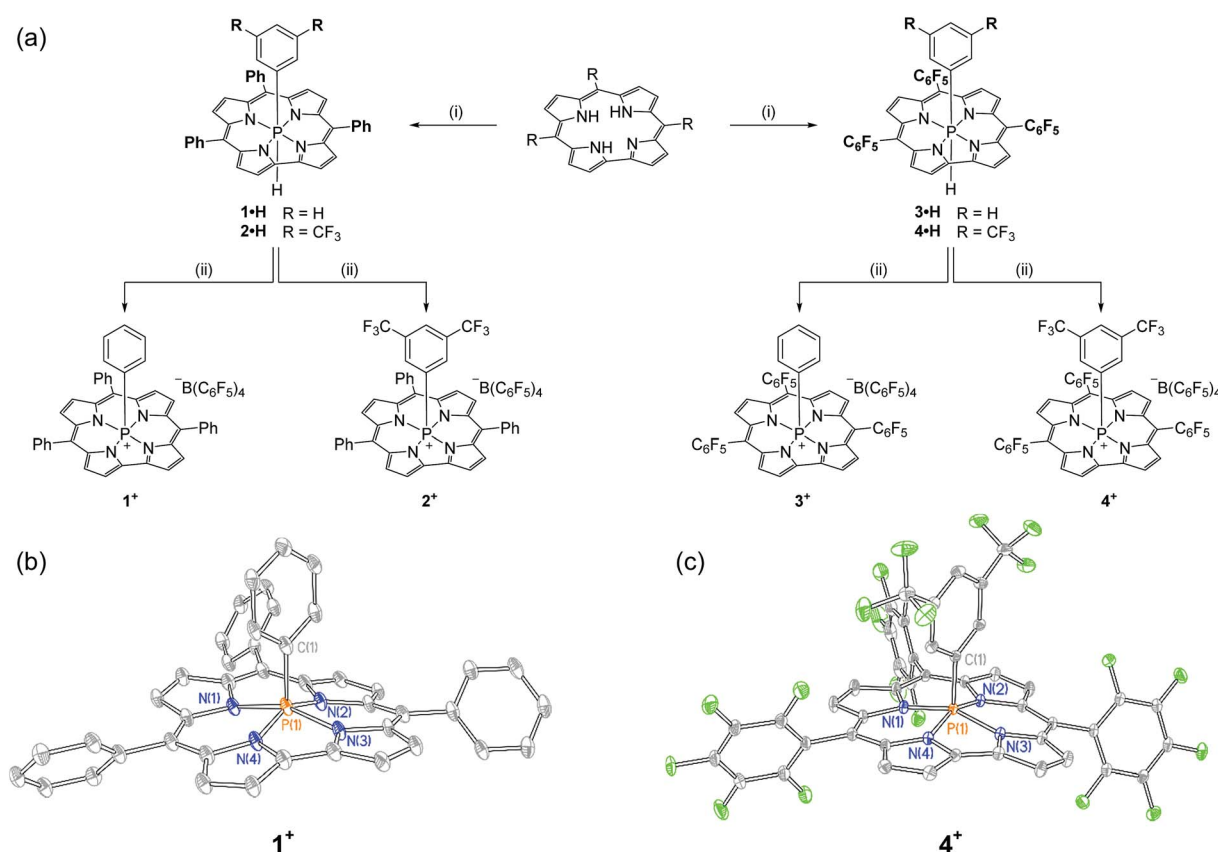
Fig. 1 (a) Synthetic path to phosphacorroles 1 + – 4 + . (i) PhPCl 4 or 3,5-(CF 3 ) 2 C 6 H 3 PCl 4 , Et 3 N, PhMe, Δ, 1 h; [Bu 4 N][BH(OAc) 3 ], PhMe, RT, overnight (ii) [Ph 3 C][B(C 6 F 5 ) 4 ], CH 2 Cl 2 , RT, 5 min. (b) X-ray structure of 1 + . Counterions and hydrogen atoms are omitted for clarity. Thermal ellipsoids are rendered at the 50% probability level. Selected bond lengths [Å], angles [°], and dihedrals [°]: P(1)–N avg 1.804(6), P(1)–C(1) 1.819(3), N(1)–P(1)–N(3) 158.1(1), N(2)–P(1)–N(4) 152.9(1), N(1)–N(2)–N(3)–N(4) –3.38(1). (c) X-ray structure of 4 + . Counterions and hydrogen atoms are omitted for clarity. Thermal ellipsoids are rendered at the 50% probability level. Selected bond lengths [Å], angles [°], and dihedrals [°]: P(1)–N avg 1.792(3), P(1)–C(1) 1.817(2), N(1)–P(1)–N(3) 158.21(7), N(2)–P(1)–N(4) 155.48(2), N(1)–N(2)–N(3)–N(4) 1.90(1).
