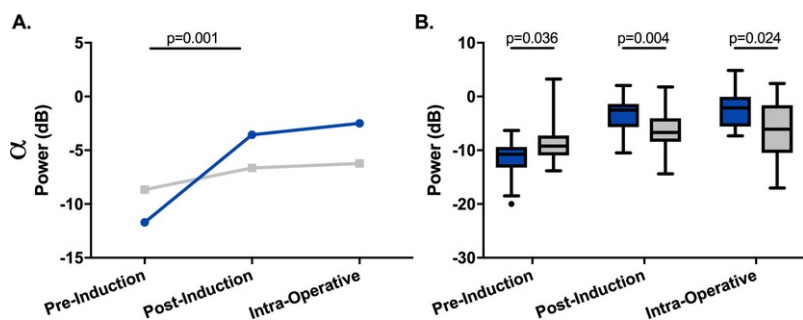
Fig. 4 Dynamics of \alpha -power from Pre- to Post-Induction and Intra-Operative state in Mid (blue) and noMid (grey) patients. (A) The graphs show the change of power within different frequency bands at pre- and at post-induction state. The increase of frontal \alpha -power from Pre- to Post-Induction was significantly stronger in Mid patients. (B) Boxplots depicting power within the \alpha -band at Pre-Induction, Post-Induction and Intra-Operative state. (For interpretation of the references to colour in this figure legend, the reader is referred to the web version of this article.)
