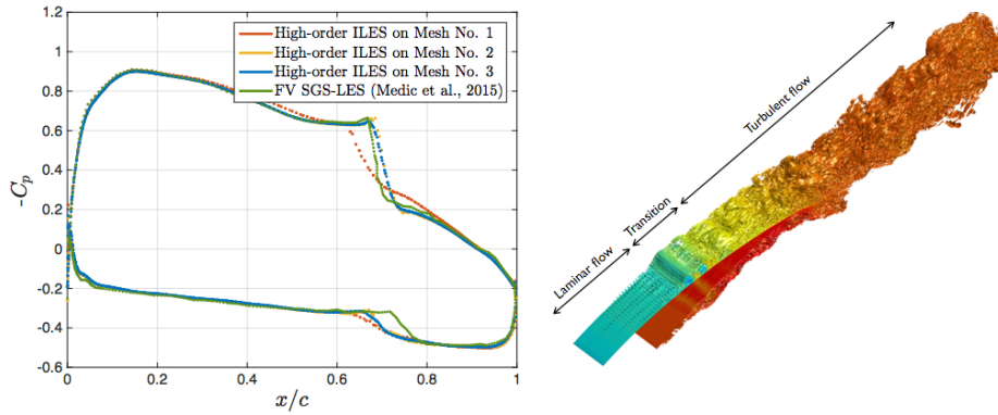
Figure 4: Negative spanwise- and time-averaged pressure coefficient computed with high-order ILES and second-order FV SGS-LES for NACA 65-(18)10 in design condition. Iso-surface of the Q-criterion [21] colored by pressure is shown on the right.
