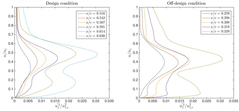
Figure 10: Transition from TS to KH modes along the separated, suction side boundary layer for NACA 65-(18)10 in design (left) and off-design (right) conditions.
