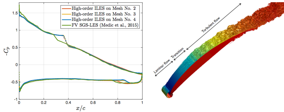
Figure 5: Negative spanwise- and time-averaged pressure coefficient computed with high-order ILES and second-order FV SGS-LES for NACA 65-(18)10 in off-design condition. Iso-surface of the Q-criterion [21] colored by pressure is shown on the right.
