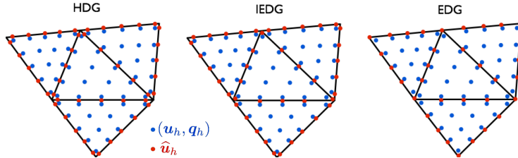
Figure 1: Illustration of the degrees of freedom for the HDG method, the IEDG method, and the EDG method. The blue nodes represent the degrees of freedom of the approximate solution (\mathbf{u}_h, \mathbf{q}_h) , while the red nodes represent the degrees of freedom of the approximate trace \widehat{\mathbf{u}}_h .
