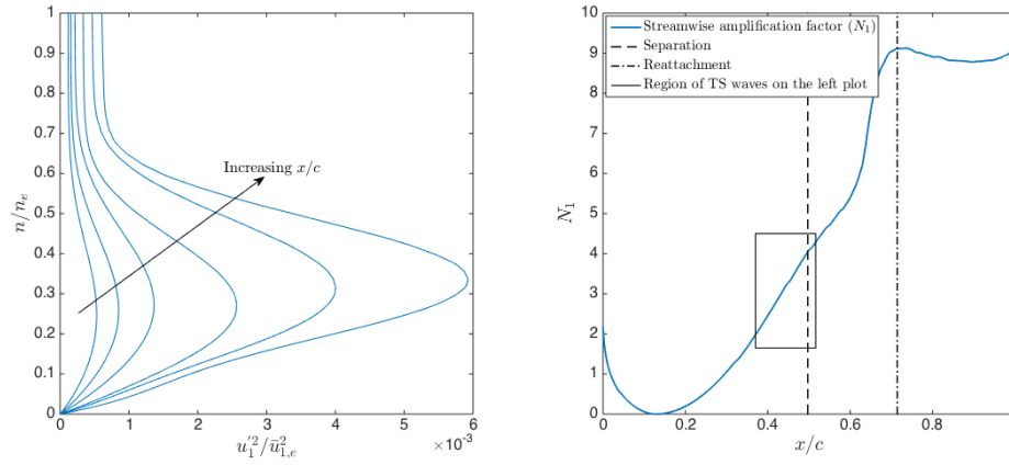
Figure 9: TS waves (left) and streamwise amplification factor (right) on the suction side for NACA 65-(18)10 in design condition. The box on the right figure indicates the region of the BL in which the TS waves on the left are located.
