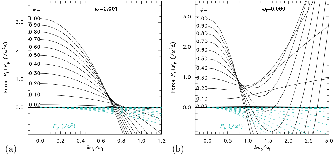
Figure 3: Total particle force F_t + F_p , and electric force F_E , normalized to \omega^2 versus wavenumber k . The dispersion relation is F_t + F_p = F_E .
