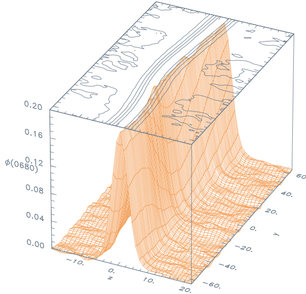
Figure 1: Two-dimensional (z, y) rendering and contours of potential \phi of an initially one-dimensional hole in the early stages of a transverse instability in a PIC simulation.
