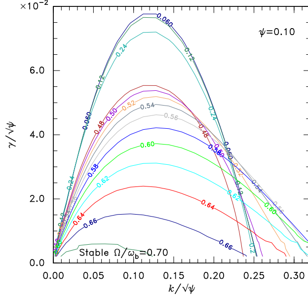
Figure 6: The zero contours of F_p + F_t - F_E for magnetized holes labeled with the increasing values of \Omega/\omega_b . The contours give the the dispersion relation \gamma(k) . Magnetic stabilization of the transverse instability occurs as \Omega/\omega_b \simeq 0.7 is approached.
