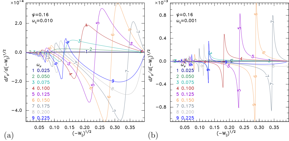
Figure 7: Contributions to the trapped particle force for specific real and imaginary parts of \omega' , as a function of trapped energy. The real part \omega_r corresponds to \Omega . The effects of bounce resonances dominate the variation at higher \omega_r . Resonances are sharper at lower \omega_i , (b), than at higher, (a).
