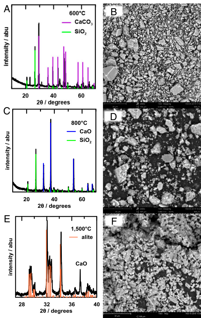
Fig. 7. Synthesis of alite using \text{CaCO}_3 and \text{SiO}_2 shows lower reactivity than with \text{Ca(OH)}_2 . After heating to 600^\circ\text{C} for 2 h in air, (A) XRD pattern and (B) SEM image show that \text{CaCO}_3 has not yet decomposed to \text{CaO} . After heating to 800^\circ\text{C} for 2 h in air, the XRD pattern (C) shows that \text{CaCO}_3 has decomposed to \text{CaO} but has not yet reacted with \text{SiO}_2 to form the alite phase. (D) SEM image of resulting \text{CaO} and \text{SiO}_2 powder mixture. After firing to 1,500^\circ\text{C} for 2 h in air, the XRD pattern (E) shows a mixture of alite with some residual \text{CaO} . (F) SEM image of this incompletely reacted mixture.
