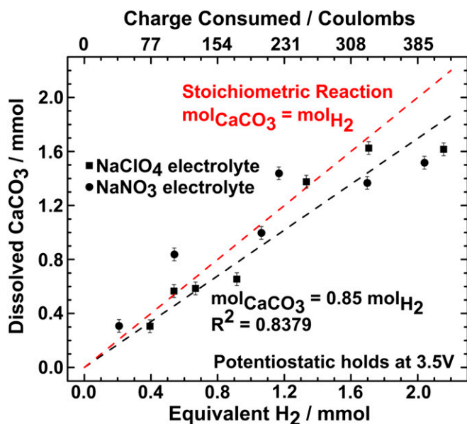
Fig. 5. Coulombic efficiency of the decarbonation reactor, measured from 13 experiments each starting with a freshly assembled H-cell of type in Fig. 2. Mass loss of \text{CaCO}_3 due to dissolution is plotted vs. total charge passed through system (top abscissa) and equivalent moles of hydrogen produced at cathode (lower abscissa), calculated assuming all current goes toward electrolysis. The red dashed line represents the stoichiometric reaction giving maximum conversion efficiency on a charge basis, and the black dashed line represents a least-squares fit to the data, the slope of which corresponds to ~85% coulombic efficiency.
