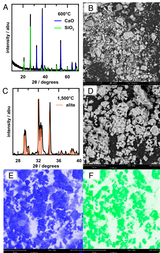
Fig. 6. Synthesis of alite, 3\text{CaO-SiO}_2 , using \text{Ca(OH)}_2 produced in decarbonation reactor. (A) XRD pattern and (B) SEM image of mixture of \text{Ca(OH)}_2 and \text{SiO}_2 after heating to 600 °C for 2 h in air. The \text{Ca(OH)}_2 has decomposed to CaO but has not yet reacted with the \text{SiO}_2 to form the alite phase. After firing at 1,500 °C for 2 h, (C) XRD pattern shows single-phase alite, the morphology of which is shown in the SEM image in D. Composition maps (E and F) of calcium and silicon, respectively, show uniform distribution of both elements.
