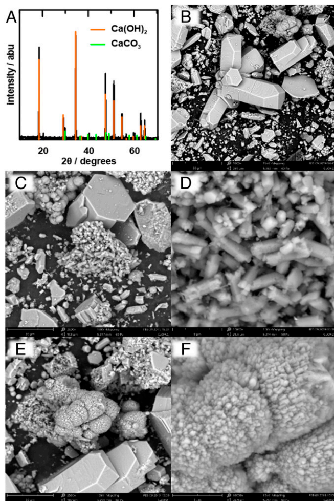
Fig. 4. \text{Ca(OH)}_2 powder produced by decarbonation reactor. (A) Powder XRD pattern from typical sample; Rietveld refinement shows 94% \text{Ca(OH)}_2 and 6% \text{CaCO}_3 . (B–F) SEM imaging shows \text{Ca(OH)}_2 crystallites of 3 length scales. (B) Largest \text{Ca(OH)}_2 crystallites have tens-of-micrometers dimensions and characteristic hexagonal-prism morphology. (C) Aggregates of smaller \text{Ca(OH)}_2 crystallites, shown at higher magnification in D , have similar hexagonal-prism morphology but are of micrometer dimensions. (E) \text{Ca(OH)}_2 with rounded nodule morphology, which at higher magnification ( F ) shows submicrometer-scale crystallites.
