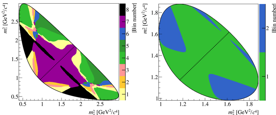
Figure 1. Binning schemes for (left) D \rightarrow K_s^0 \pi^+ \pi^- decays and (right) D \rightarrow K_s^0 K^+ K^- decays. The diagonal line separates the positive and negative bins, where the positive bins are in the region in which m_-^2 > m_+^2 is satisfied.
