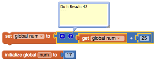
Figure 9. Invoking DoIt on an expression block displays the value of that block, as calculated by the interpreter on the device.
