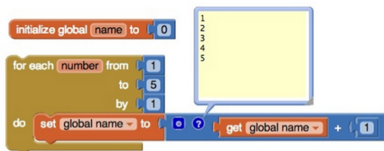
Figure 10. Selecting Watch on an expression within a loop shows all values of that expression when the loop is executed.
