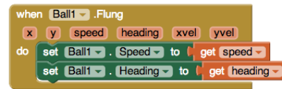
Figure 3. Blocks event handler for flinging Ba111 .
