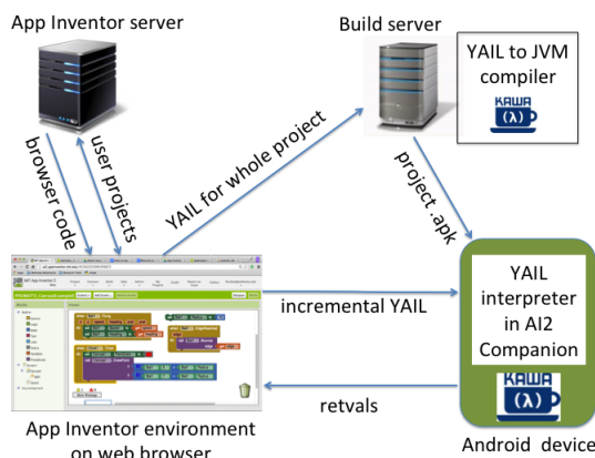
Figure 7. The key elements and interactions in the App Inventor system. The browser and Android device are assumed to be connected and communicating as explained in Sec. 4.
