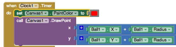
Figure 5. An event handler that draws a red dot at Ba111 ’s center every time the timer fires.
