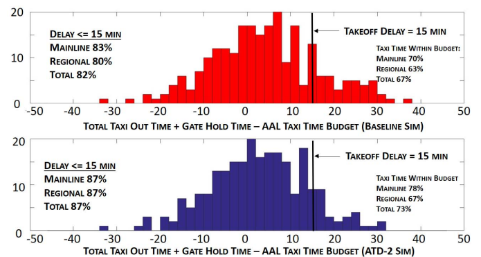
Figure 5. ATD-2 system had a beneficial impact on the airport's on-time performance as per an analysis of Total Taxi-out Times as compared to Taxi-Out Time budgets
