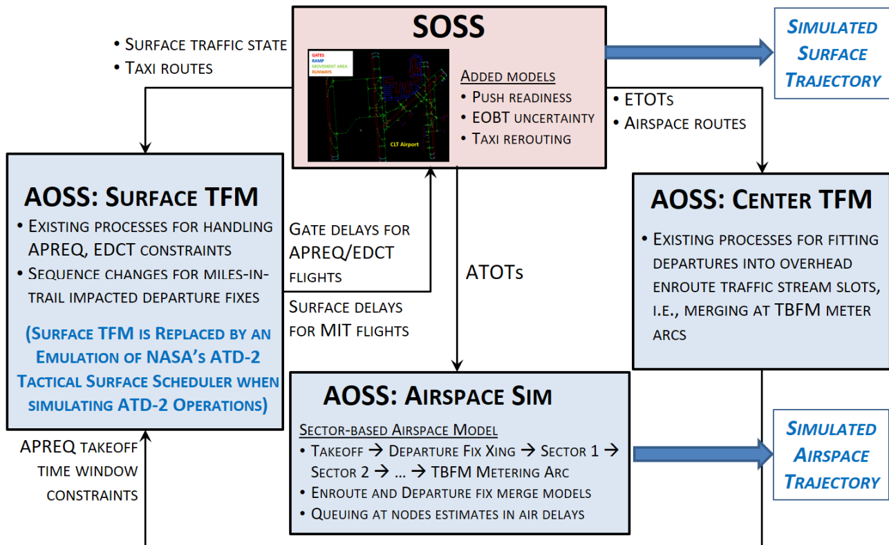
Figure 1. Integrated Surface Airspace Simulation Environment
