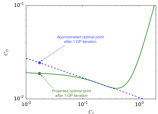
Fig. 3 Signomial equality constraint C_D = f(C_L) and its approximation.
