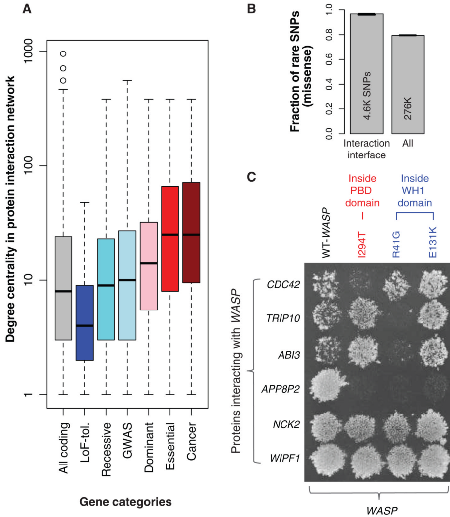
Fig. 3. SNPs in protein-protein interaction (PPI) network
