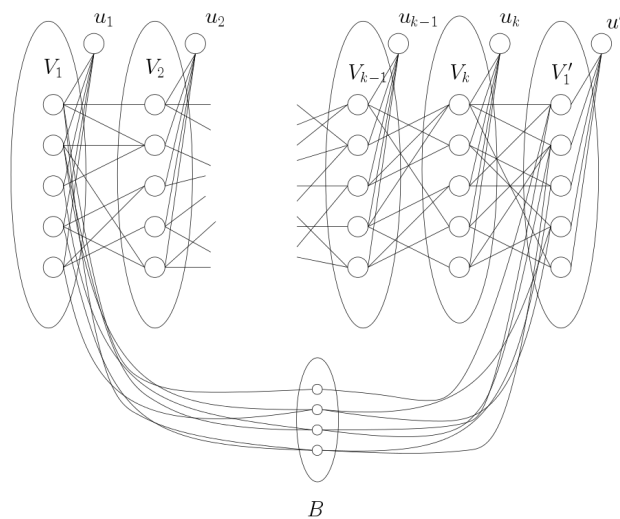
Figure 5: The Wiener Index gadget.
