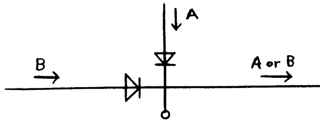
The OR Function
