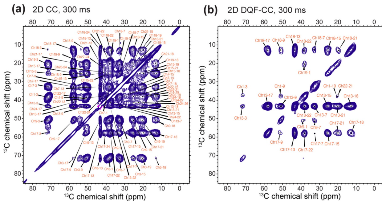
Figure 3. 300 ms (a) 2D CC spectrum and (b) 2D DQF-CC spectrum of 1- ^{13}\text{C} CHOL in POPC/POPG membranes, showing full assignment of the intramolecular CHOL cross peaks. The spectra were measured at \sim 110 K with DNP.
