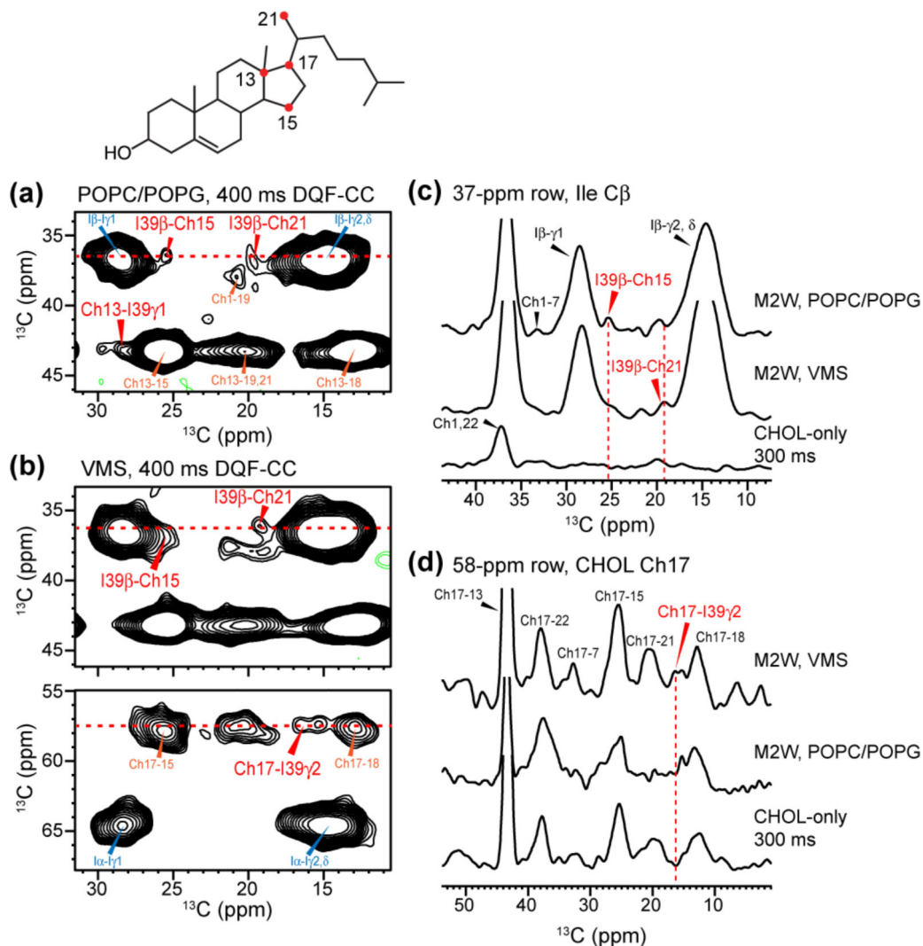
Figure 6. Protein-cholesterol correlations observed in DNP 2D DQF-CC spectra of GI-M2W(22–61) peptide in two lipid membranes. (a) Regions of the 400 ms 2D DQF-CC spectrum of GI-M2W in POPC/POPG membranes. (b) Regions of the 400 ms 2D DQF-CC spectrum of GI-M2W in the VMS membranes. I39 cross peaks with several CHOL carbons are detected. (c) 1D cross sections extracted from the I39 C \beta chemical shift, showing similar cross peaks in the two lipid membranes. (d) 1D cross sections extracted from the CHOL Ch17 chemical shift, showing a protein-cholesterol cross peak in the VMS membrane but not the POPC/POPG membrane.
