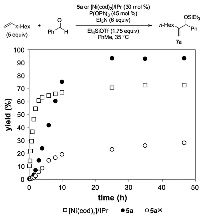
Figure 1. Product profile for the nickel catalyzed carbonyl-ene reaction with [\text{Ni}(\text{cod})_2]/\text{IPr} or 5a . Yields determined by GC against a calibrated internal standard (dodecane, 10 mol %). [a] The addition of cod (0.6 equiv) was used.
