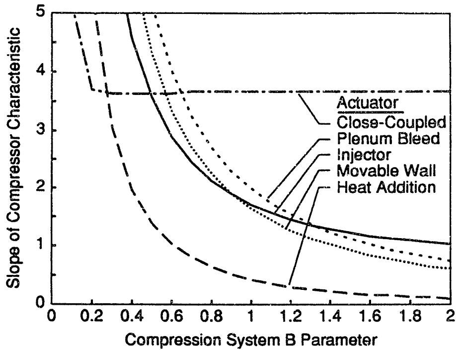
Figure 6-3: Maximum slope at which the RMS actuation will be no greater than 25% of the maximum actuator authority
