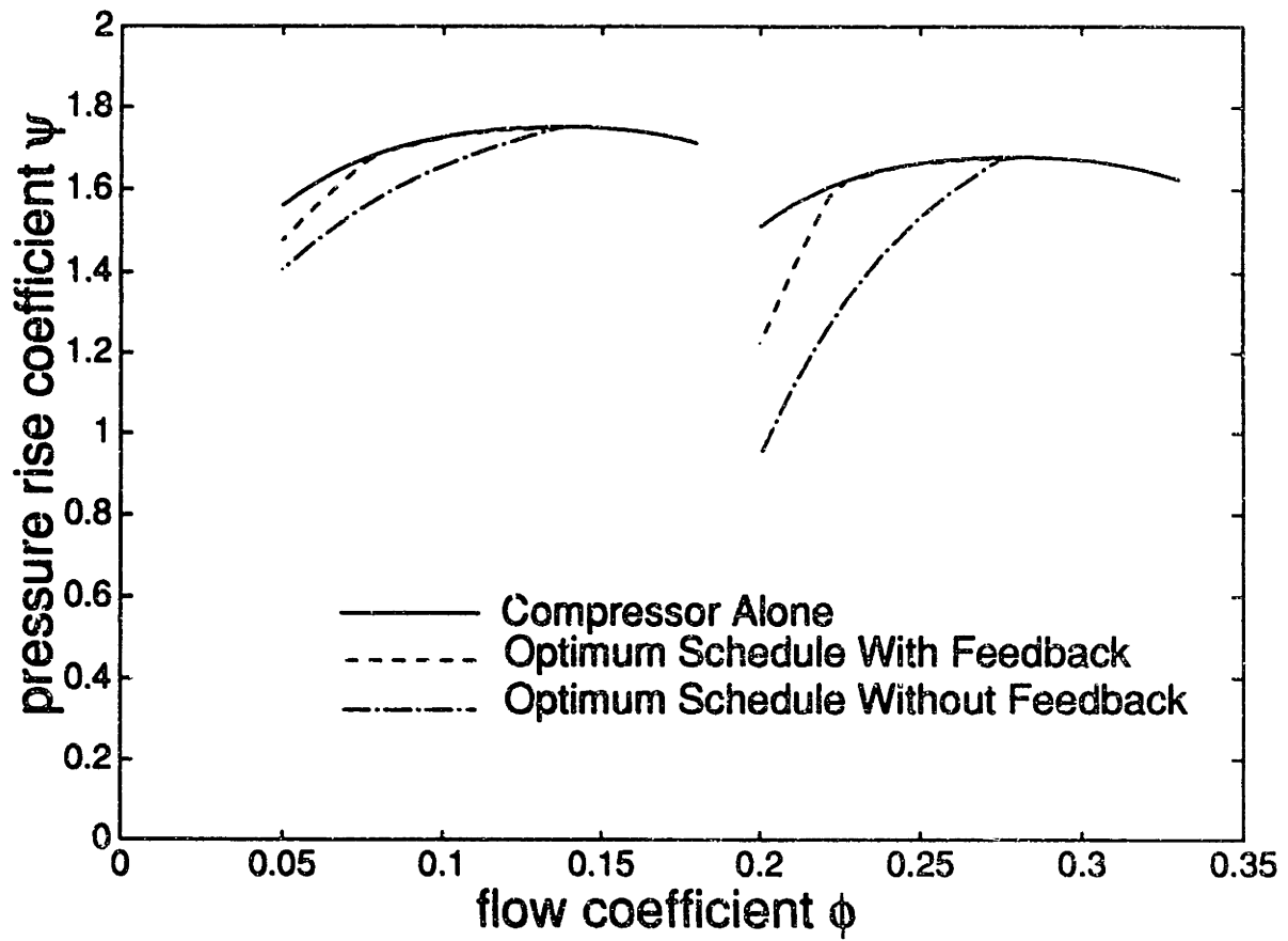
Figure 7-5: Effect of flow rate on optimal scheduled performance similar compressor characteristics
