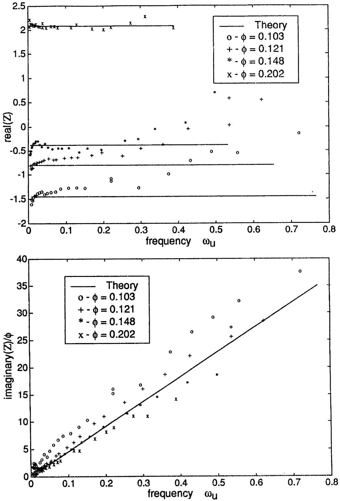
Figure 4-6: Comparison of experimentally determined compressor impedance with quasi-steady theory
