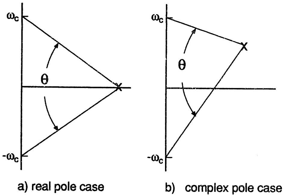
Figure 5-7: Geometrical Construction for the weighting function \theta(\omega_c) a) real pole b) complex conjugate pole
