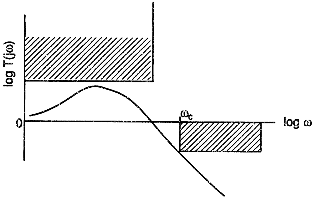
Figure 5-6: Typical frequency domain performance specification for the complementary sensitivity transfer function
