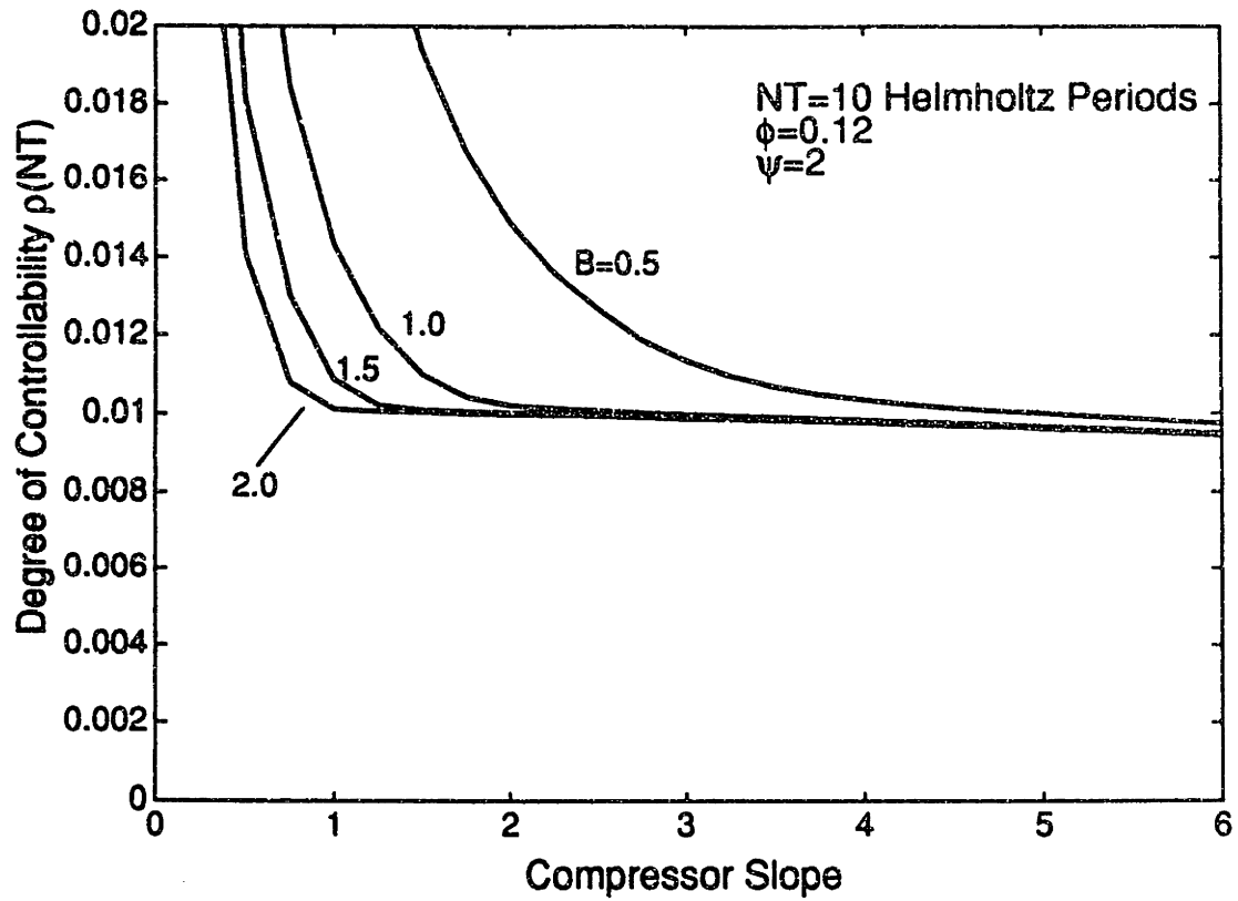
Figure 5-4: Degree of Controllability as function of system parameters for close-coupled actuator
