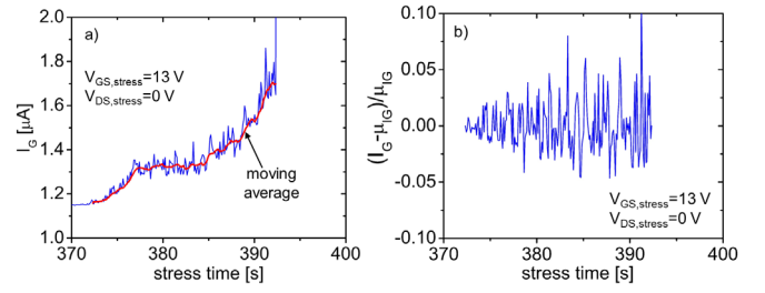
Fig. 12. Progressive breakdown noise analysis illustrated for a breakdown experiment at T=150^\circ\text{C} . a) A moving average \mu_{IG} of the gate current is obtained during progressive breakdown. This gives the background gate leakage current during PBD, \mu_B . b) Average I_G is subtracted from the gate current, leaving only the noise component. The data is then normalized by the average gate current to account for differences in background leakage at different temperatures (Fig. 3).
