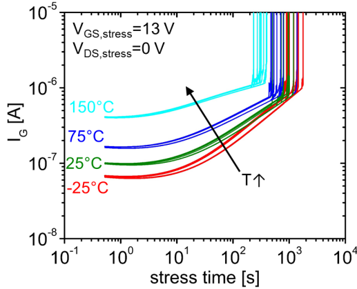
Fig. 3. Gate current I_G as a function of stress time during a series of constant V_{GS, stress} experiments for different temperatures (10 devices at each temperature). The FETs are held at V_{GS, stress}=13 V until the gate dielectric breaks down. As the stress temperature increases, I_G increases as well. PBD is visible near the end of the TDDB experiments.
