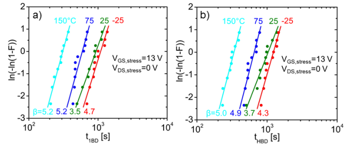
Fig. 5. Weibull plots of a) t_{1BD} and b) t_{HBD} at four different temperatures: 150, 75, 25, and -25^\circ\text{C} . V_{GS, stress}=13 V, V_{DS, stress}=0 V. As the temperature increases, time-to-breakdown decreases. The slope of each set of breakdown statistics, \beta , is shown at the bottom of each graph.
