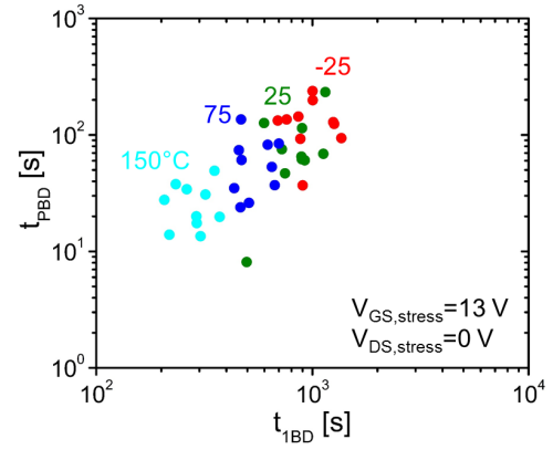
Fig. 8. PBD time versus time-to-first-breakdown t_{1BD} for all 40 samples in Fig. 3 stressed at V_{GS, stress}=13 V and V_{DS, stress}=0 V at different temperatures. The data show that t_{1BD} and t_{PBD} are uncorrelated. As temperature increases both t_{1BD} and t_{PBD} decrease.
