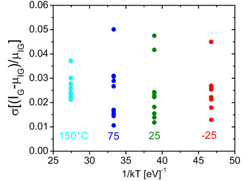
Fig. 13. Standard deviation of the normalized noise on the gate current I_G during progressive breakdown. No real trend is observed as a function of temperature, suggesting that the underlying mechanism for the PBD noise may be a tunneling phenomenon.
