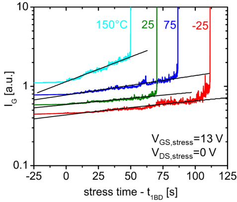
Fig. 10. Gate current I_G evolution for a typical constant-voltage TDDB experiment at each temperature: 150, 75, 25, and -25^\circ\text{C} . x-axis is shown as stress time - t_{1BD} so that 1BD begins at 0 s. I_G data at different temperatures have been shifted to arbitrary units (a.u.) such that I_G evolution at each temperature is separable and visible. Also shown is an exponential fit for the progressive breakdown regime, fit to the form I_{G1} \cdot \exp([t-t_{1BD}]/\tau_{PBD}) , where I_{G1} is the gate current at first breakdown, and t_{1BD} is the time at which 1BD occurs.
