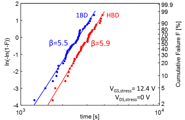
Fig. 2. Weibull plot of t_{1BD} and t_{HBD} . V_{GS, stress}=12.4 V, V_{DS, stress}=0 V at RT. Nearly parallel statistics for time-to-first breakdown 1BD and HBD suggest a unified degradation mechanism.
