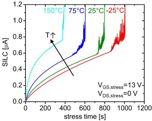
Fig. 4. Stress-induced leakage current (SILC) as a function of stress time for a representative device at each temperature during a series of constant V_{GS, stress} experiments. The FETs are held at V_{GS, stress}=13 V until the gate dielectric breaks down. As the stress temperature increases, the rate of increase of SILC increases as well. This is consistent with faster rates of defect generation at higher temperatures.
