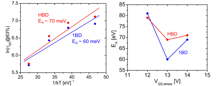
Fig. 6. a) Arrhenius plot of t_{1BD} and t_{HBD} from Fig. 4. \tau_{BD} is extracted at a cumulative device failure of F=63.2\% for every temperature. Lines drawn as guides for the eye. E_A for both 1BD and HBD are very similar, suggesting a common underlying physical mechanism. b) Activation energy as a function of V_{GS, stress} for both 1BD (blue) and HBD (red). No definitive trend is shown across the three values of V_{GS, stress} tested and E_A remains small in each case.
