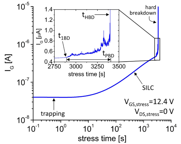
Fig. 1. Gate current I_G as a function of stress time during a constant V_{GS, stress} TDDDB experiment at RT. The MIS-HEMT is held at V_{GS, stress}=12.4 V until the device breaks down. V_{DS, stress}=0 V. The inset shows a clear onset of noise in I_G marking the beginning of the PBD regime.
