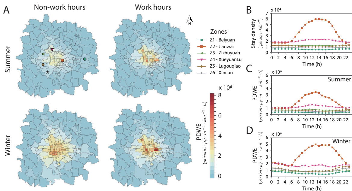
Figure 3: Population density weighted exposure (PDWE) to \text{PM}_{2.5} per zone. A Average PDWE in each zone during work (from 9:00 am to 5:00 pm) and non-work hours during the summer and winter of 2015. The zones in downtown are exposed to heavier \text{PM}_{2.5} concentration during work hours than non-work hours. B Hourly population density of six selected zones. The higher population density during daytime in Zone Z2 and Z4 captures the incoming flow during work hours. C Hourly PDWE of selected zones in the summer. D Hourly PDWE of selected zones in the winter.
