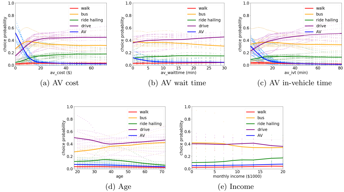
Fig. 5. Choice probability functions varying with inputs values; the curves are generated by varying the targeting input variables while holding all the other variables constant; light curves are the individual MTLDNN results; dark ones are the average of top 10 models.
