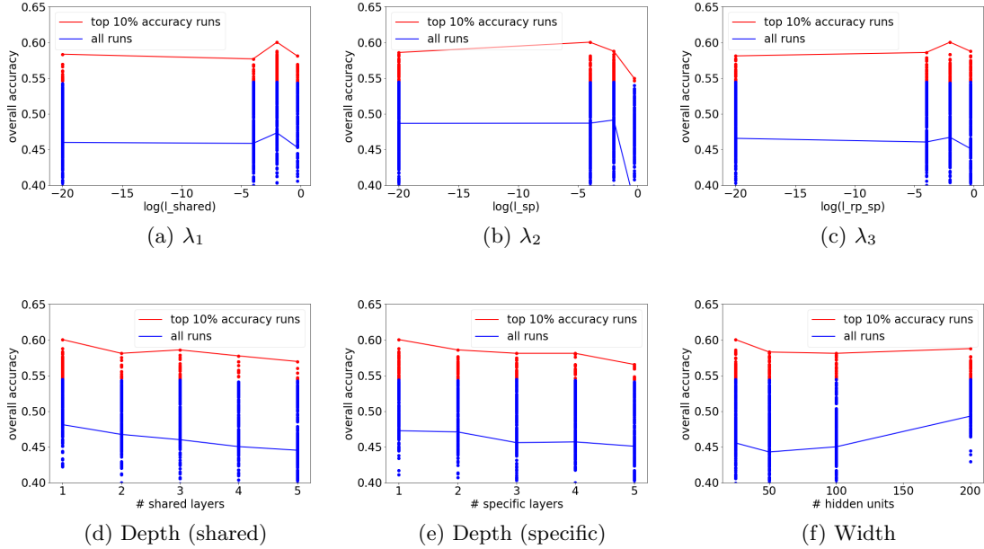
Fig. 4. Prediction accuracy with regularization and architectural hyperparameters; red and blue dots are the results of individual models; blue lines connect average prediction accuracy of all models, and red ones connect the models with the maximum prediction accuracy.
