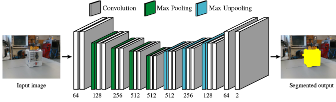
Fig. 4. Machine region segmentation network. The number below each layer indicates the dimension of corresponding feature maps.
