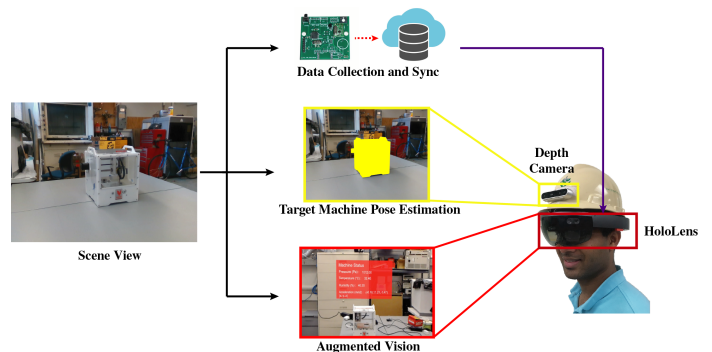
Fig. 1. Our system collects the target machine’s information in real-time and estimates its pose via a helmet-mounted depth camera. The operator can visualize accurately and precisely superimposed augmented digital information through the HoloLens.
