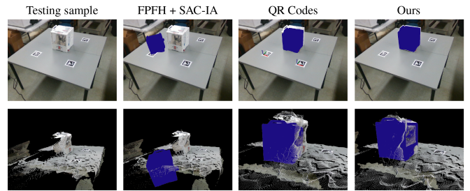
Fig. 8. Visualize pose estimation results (Top row: Project transformed the machine model onto scene images; Bottom row: Transform the machine model into scene point clouds). Note that QR codes shown in the images are only used for marker-based method.
