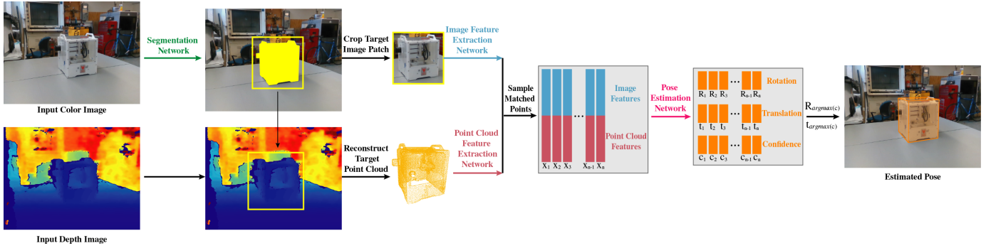
Fig. 3. Pipeline for target machine pose estimation given an input RGB-D image pair.
